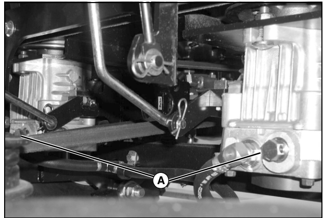
A - Hydraulic Pump Free-Wheel Valves
