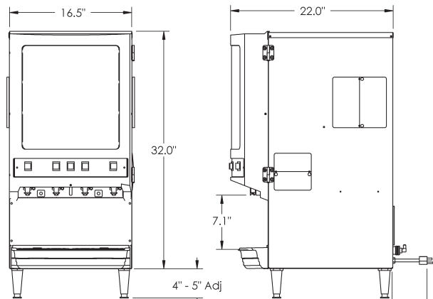
Model PIC-4W
