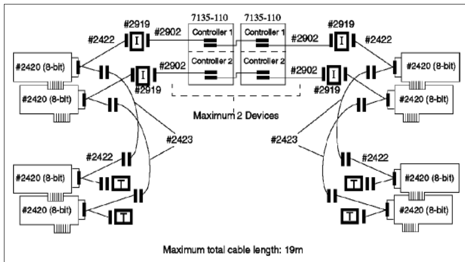
Figure 10. 7135-110 RAIDiant Arrays Connected on Two Shared 8-Bit SCSI Buses
