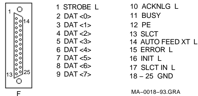
Figure B-3 Parallel Printer Port (Bidirectional)
