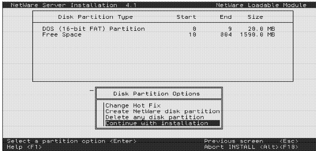
Figure 94. Create Partition
