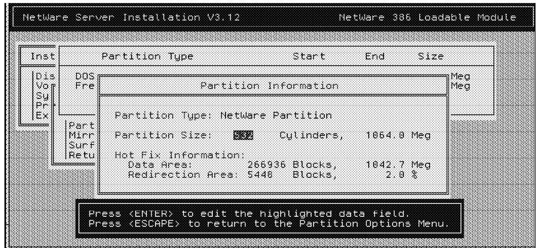
Figure 84. Partition Information
