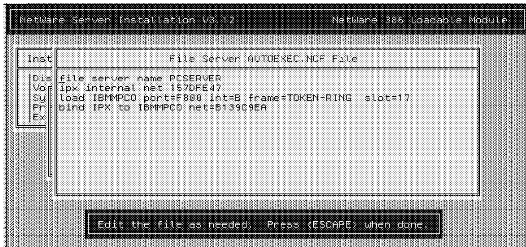
Figure 90. AUTOEXEC.NCF File
