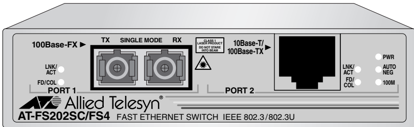
Figure 2 AT-FS202SC/FSx Series Front Panel (AT-FS202SC/FS4 Model)
