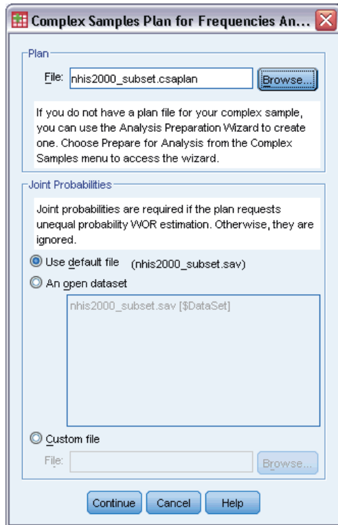
Figure 15-1 Complex Samples Plan dialog box
