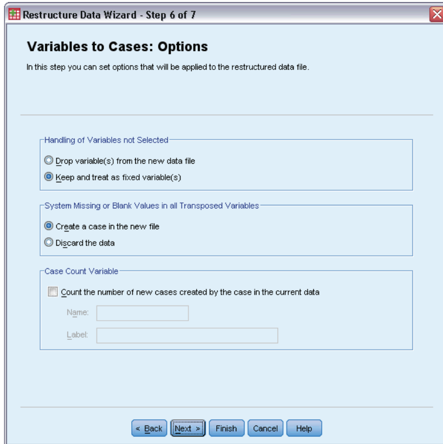
Figure 22-32 Restructure Data Wizard, Variables to Cases Create One Index Variable step
