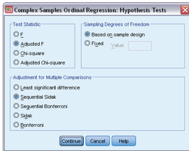
Figure 21-4 Hypothesis Tests dialog box
