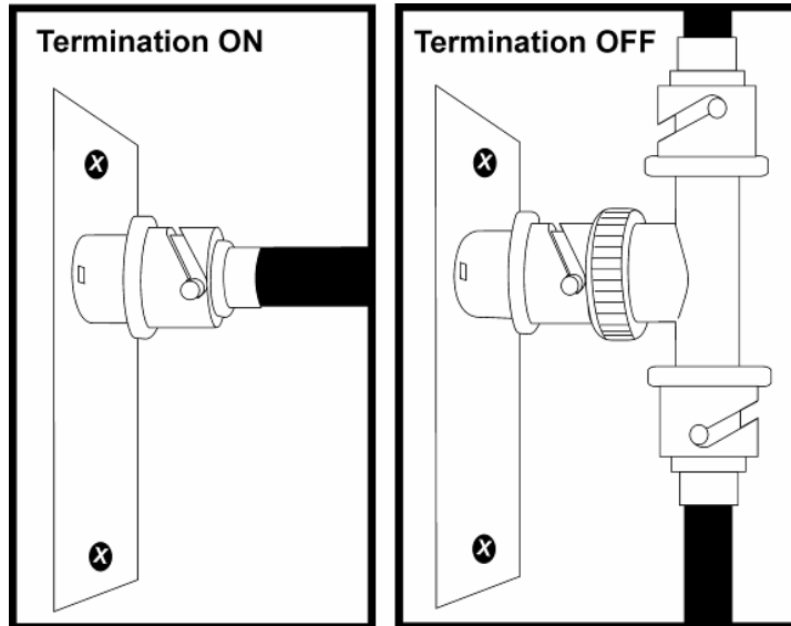
BNC Port Termination
