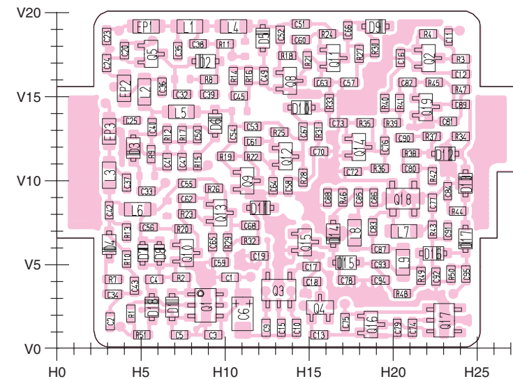
9-3 VCO BOARD • TOP VIEW
