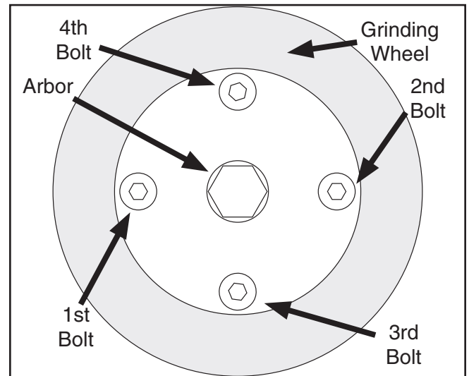
Figure 9. Wheel bolt mounting order.
