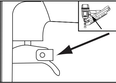
Figure 5. Single/bump fire selector.
