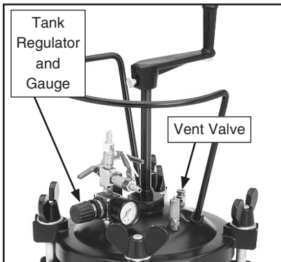
Figure 6. Regulator and vent valve.
