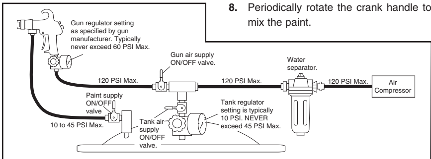
Figure 5. Paint tank connect to air compressor and spray gun.
