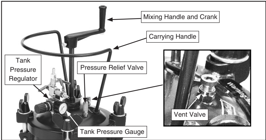
Figure 2. Controls and features.
