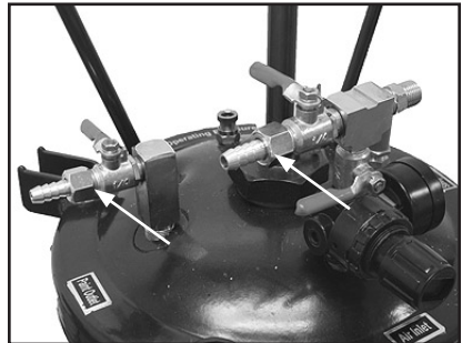
Figure 4. Spray gun fittings installed.
