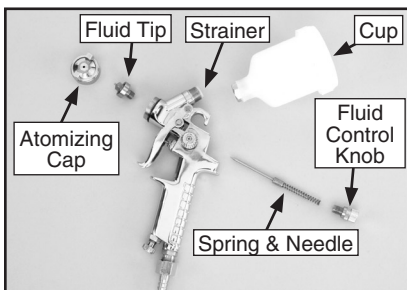
Figure 9. Disassembly for cleaning.
