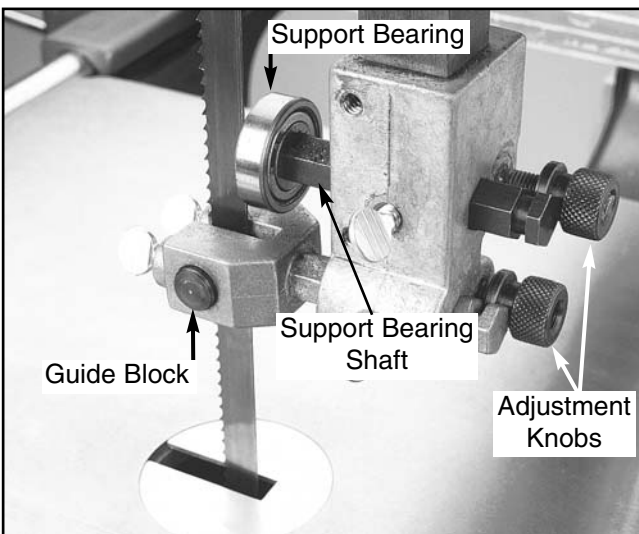
Figure 18A. Upper guide assembly.
