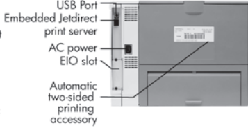
Rear view
