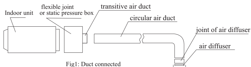
Fig1: Duct connected
