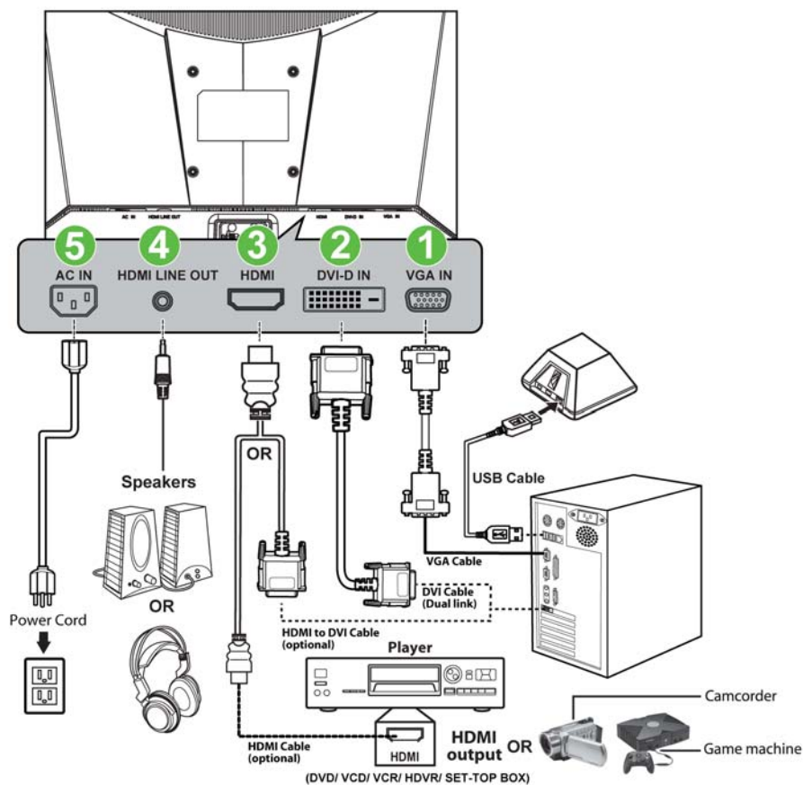
Figure.2. Connecting to a PC
