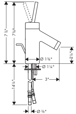
Starck single lever bidet mixer 10201XX1
