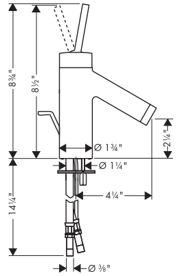
Starck single lever basin mixer 10016XX1
