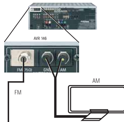
Figure 18 – Antenna Connections
