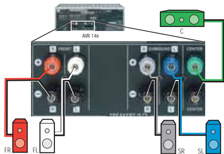
Figure 16 – Speaker Connections
