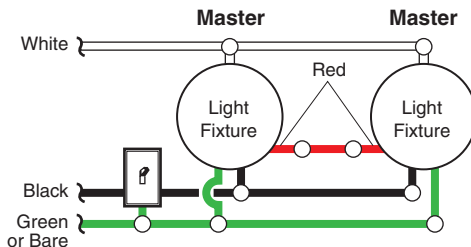
Wiring Diagram 3
