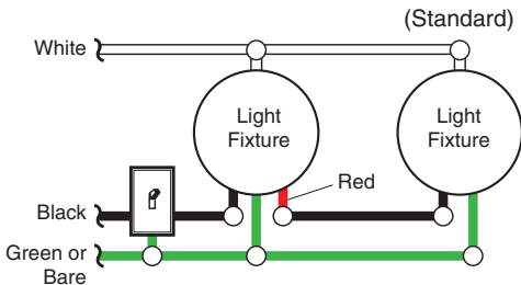
Wiring Diagram 1
