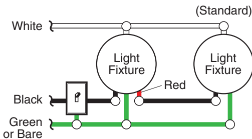
Wiring Diagram 1
