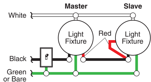
Wiring Diagram 2
