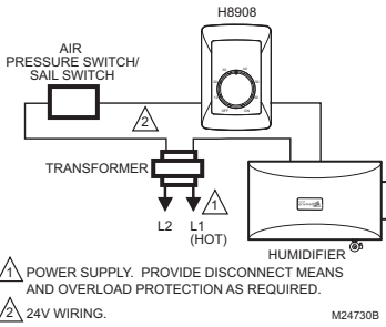
Fig. 15. Wiring H8908 in line with air pressure switch/sail switch and humidifier.
