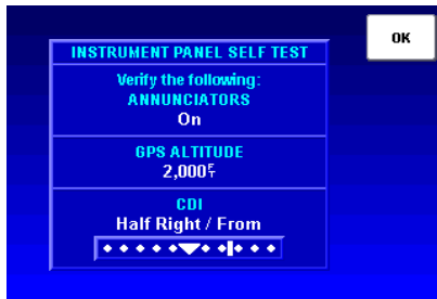
KMD 250 with Internal GPS
