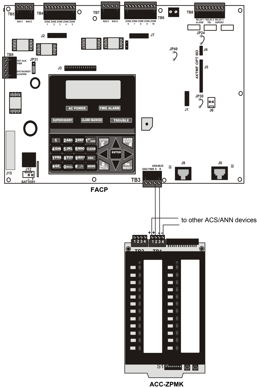
Figure D.6 Connection for MS-5UD-3/7 and MS-10UD-3/7 to ACC-ZPMK
