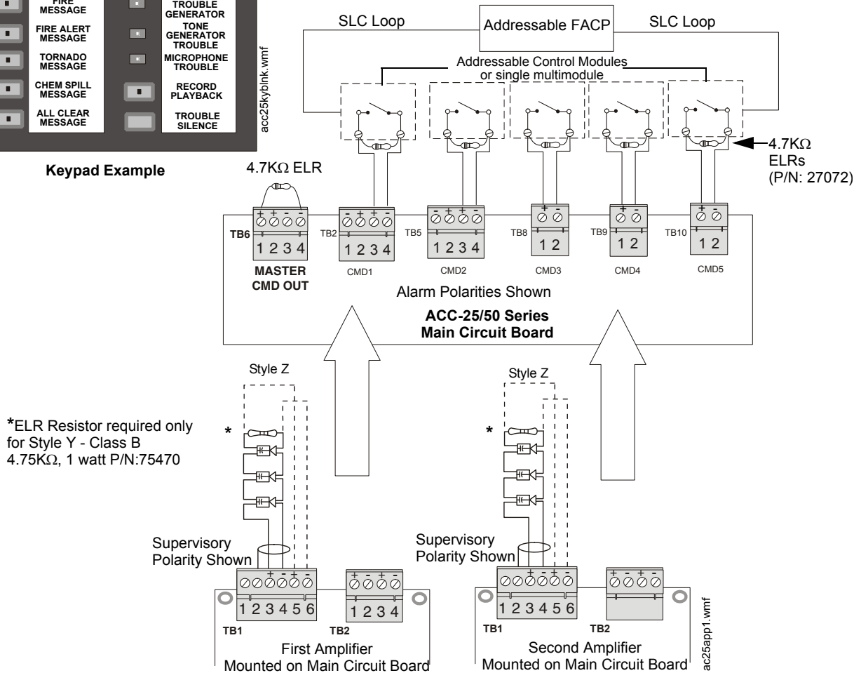
Figure 5.4 Two Speaker Circuits - Single Output Zone, Five Input Channels (five messages)
