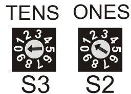
Figure 2.3 ACC-ZPMK Addressing Switches
