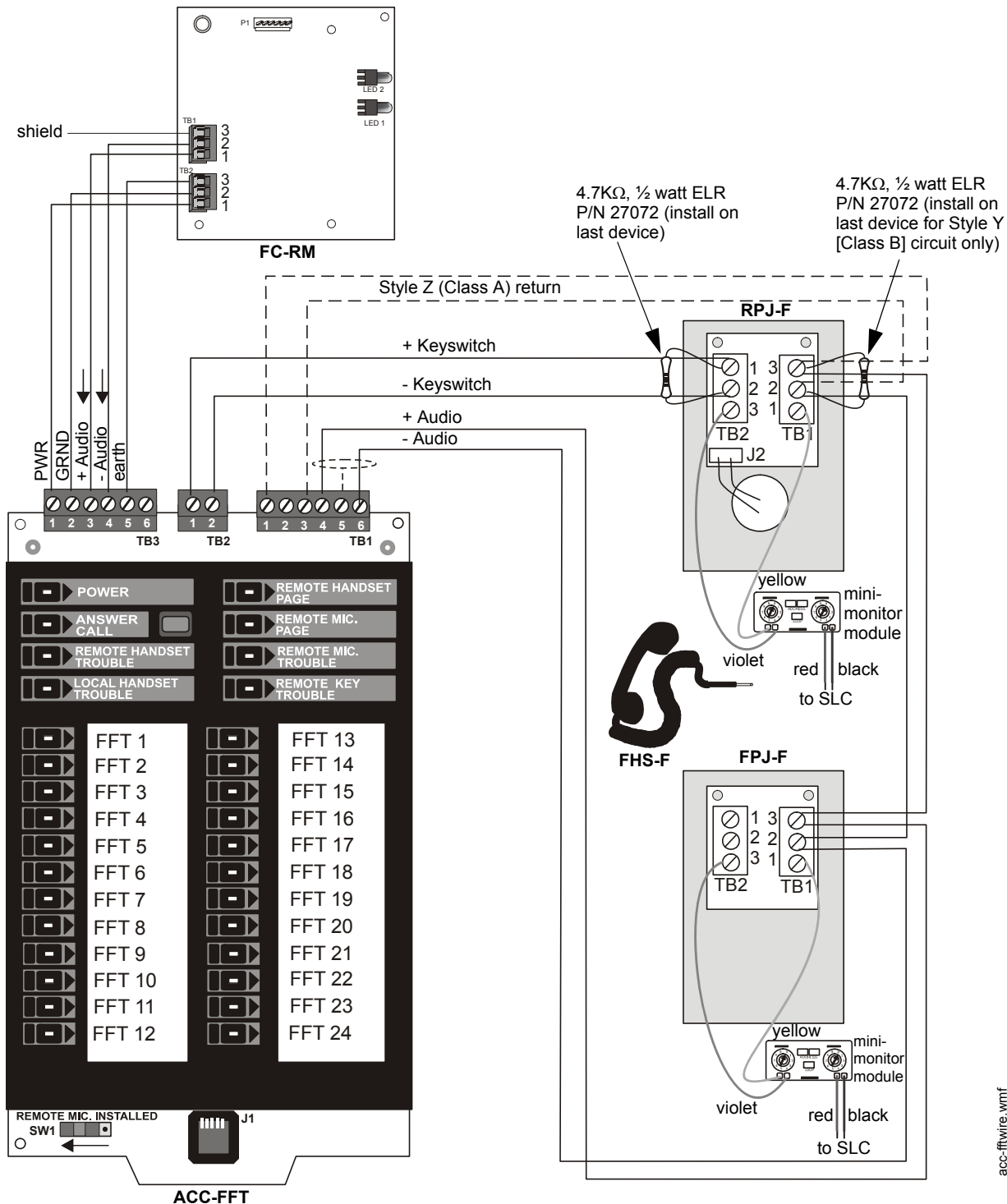
Figure 3.15 ACC-FFT Fire Fighter Telephone Module
