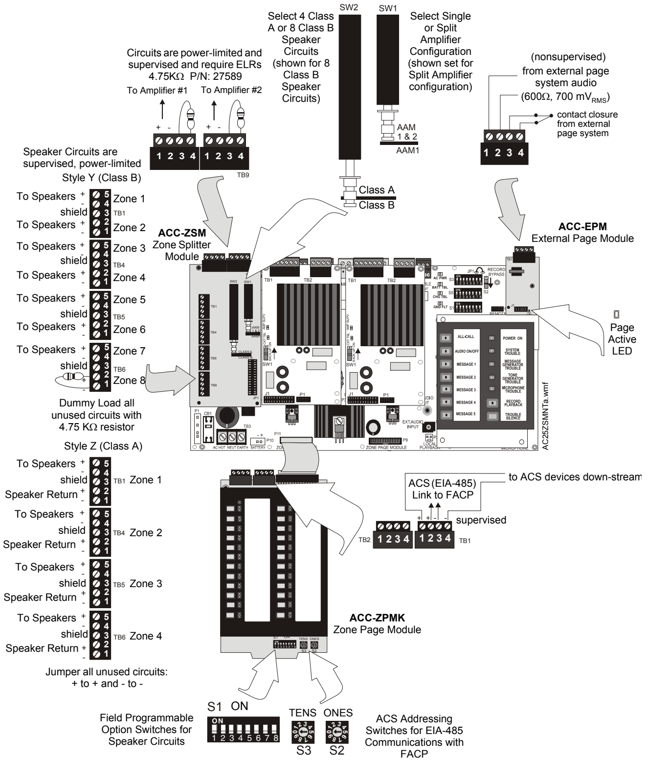
Figure 1.3 ACC-25/50ZS Main Board With Modules
