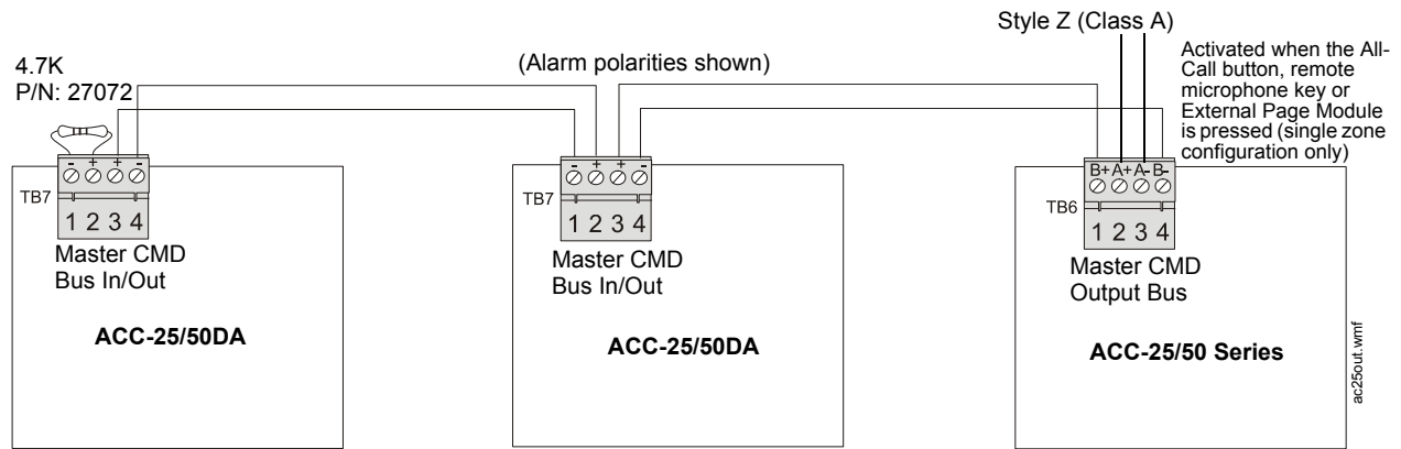
Figure 3.8 Example 1 - Activating Multiple ACC-25/50DAs with Master CMD Output Bus
