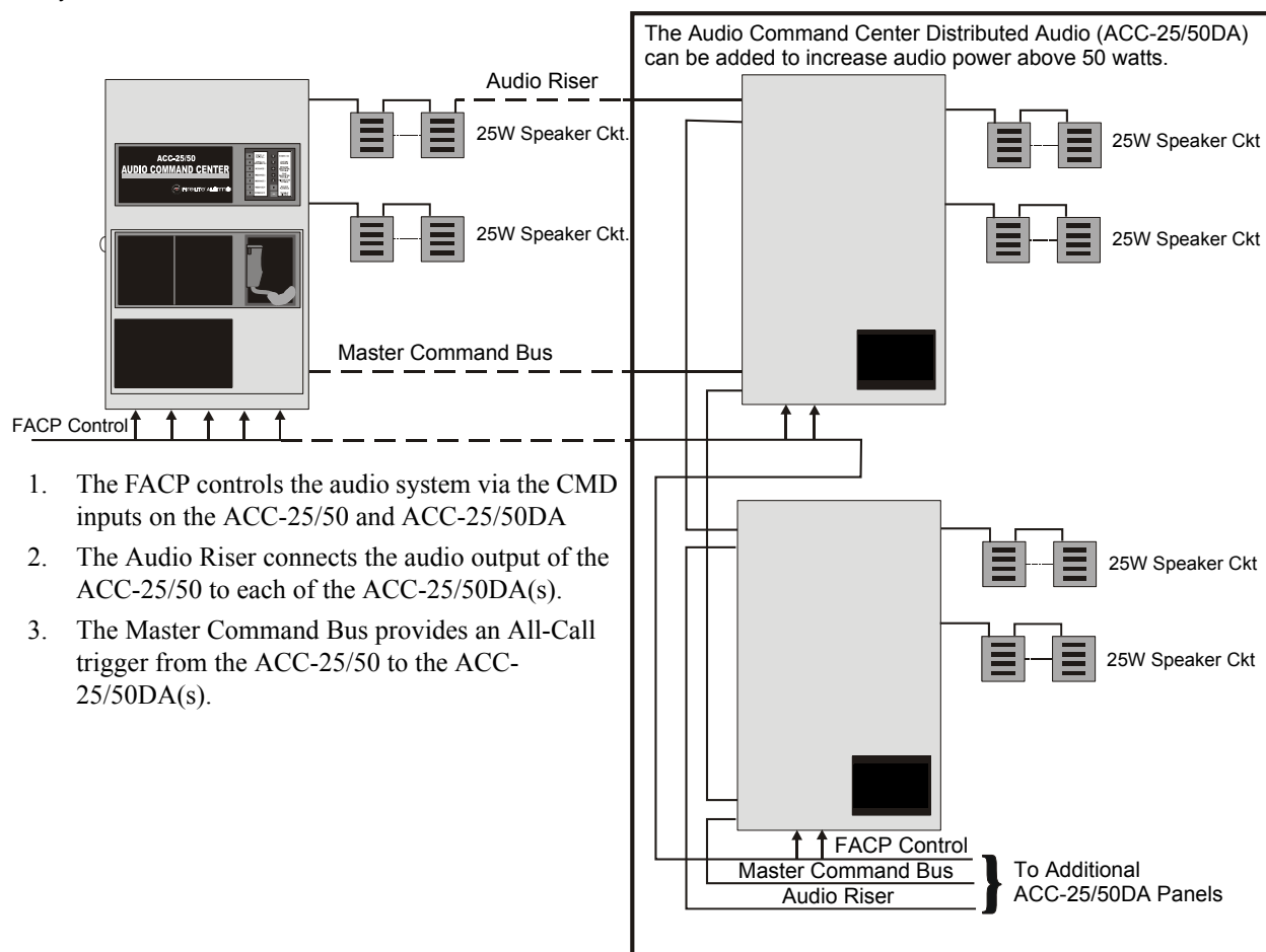
Figure 5.8 ACC-25/50 to ACC-25/50DA Connections
