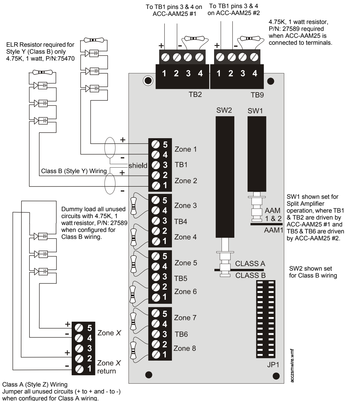
Figure 3.14 Zone Splitter Module
