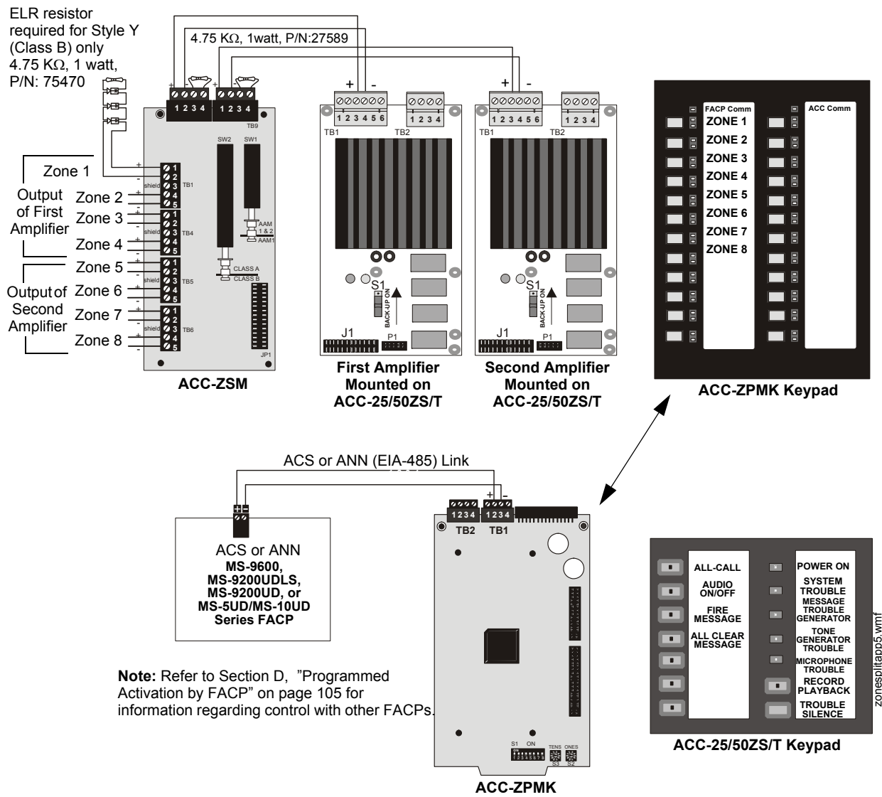
Figure 5.7 ACC-25/50ZS/T 50 Watt Zone Splitting
