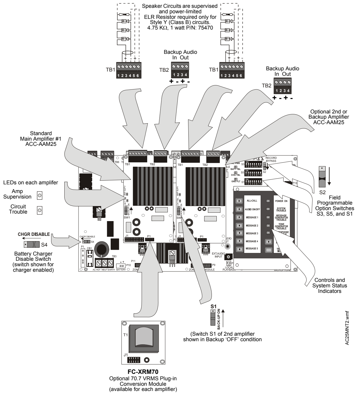
Figure 1.2 Command Board With Amplifiers
