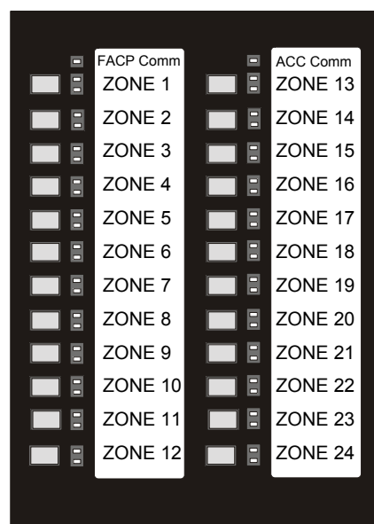
Figure 4.4 ACC-ZPMK Keypad/Annunciator
