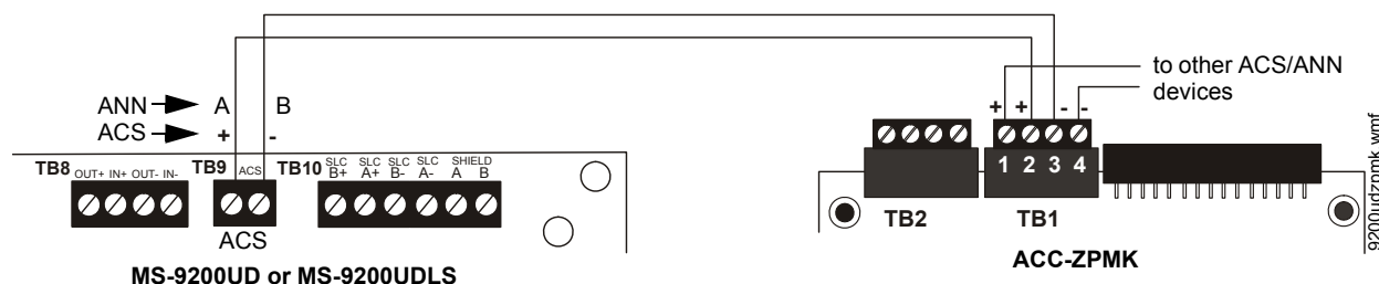
Figure D.2 Connection for MS-9200UD or MS-9200UDLS to ACC-ZPMK
