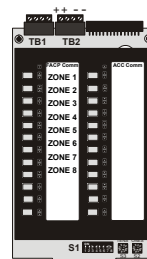
Figure D.4 ACC-25/50ZS/T Connection to ACM-8RF
