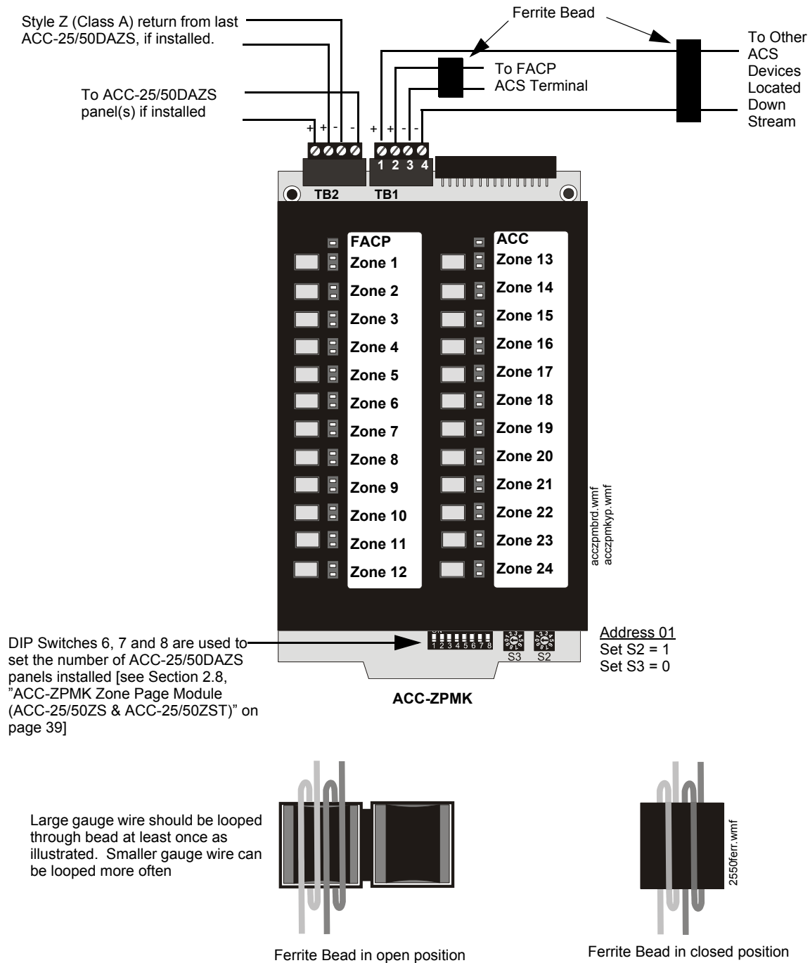
Figure 3.13 Zone Page Module
