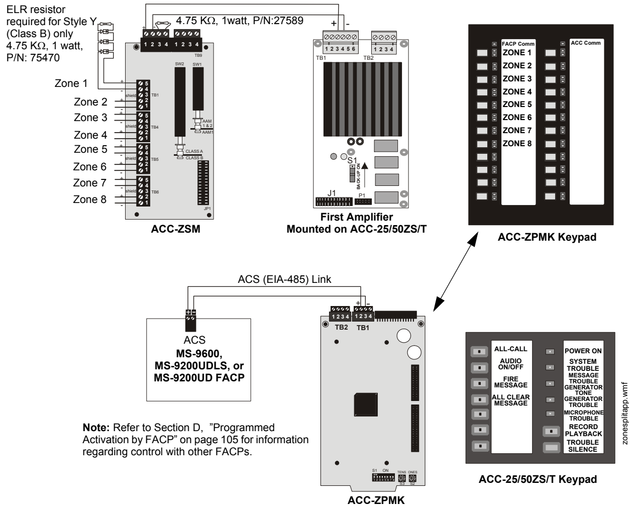
Figure 5.5 ACC-25/50ZS/T 25 Watt Zone Splitting
