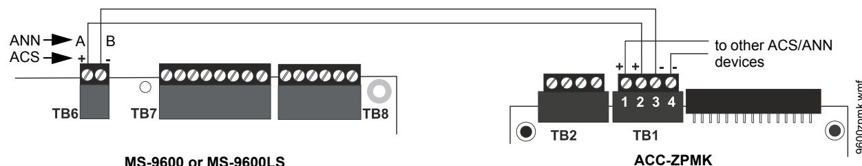
Figure D.1 Connection for MS-9600 or MS-9600LS to ACC-ZPMK
