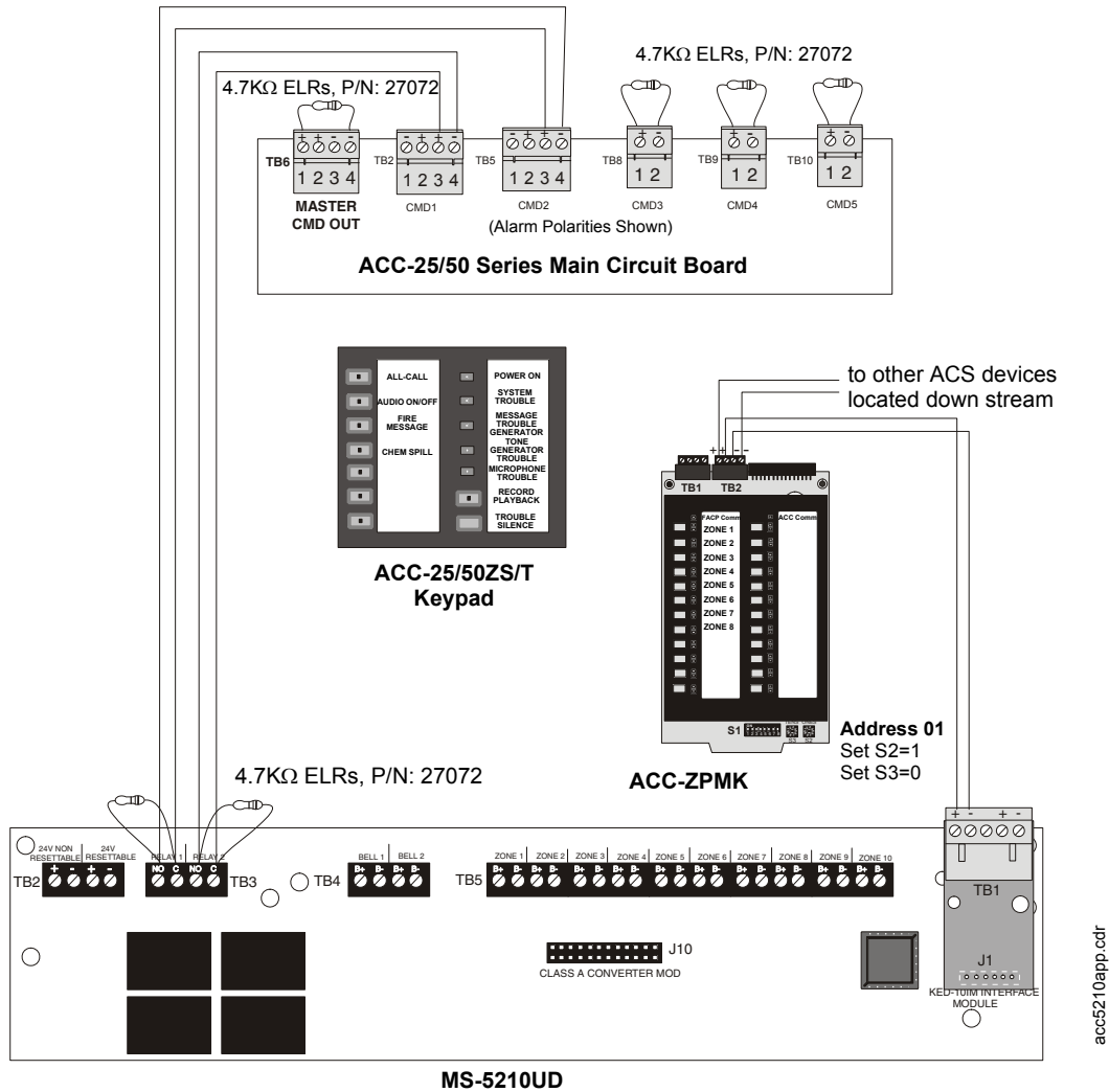
Figure D.3 MS-5210UD Connection to ACC-25/50ZS or ACC-25/50ZST
