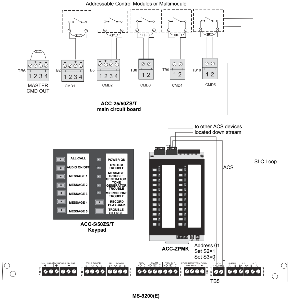
Figure D.5 ACS Connection for MS-9200(E) to ACC-ZPMK
