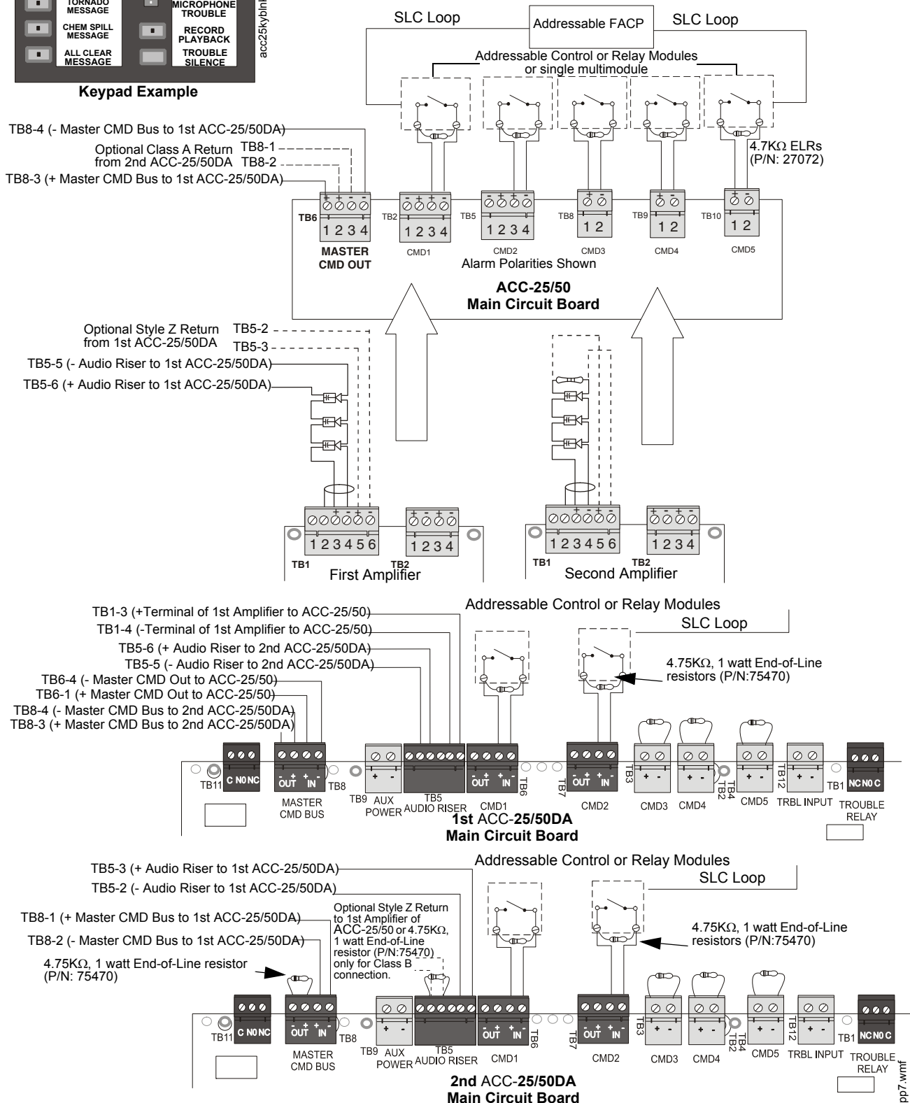
Figure 5.8 ACC-25/50 to ACC-25/50DA Terminal Connections
