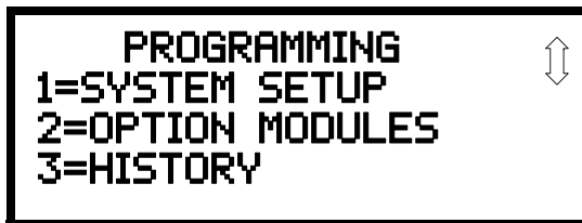
Programming Screen #2
