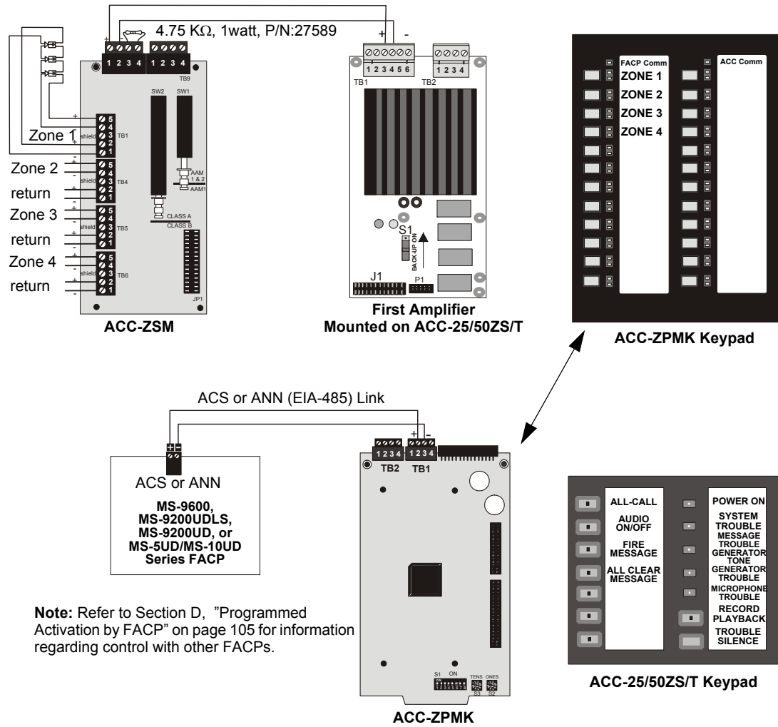
Figure 5.6 ACC-25/50ZS/T 25 Watt Zone Splitting
