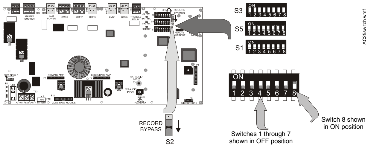
Figure 2.1 Field Programming DIP Switches for ACC-25/50, ACC-25/50ZS, & ACC-25/50ZST
