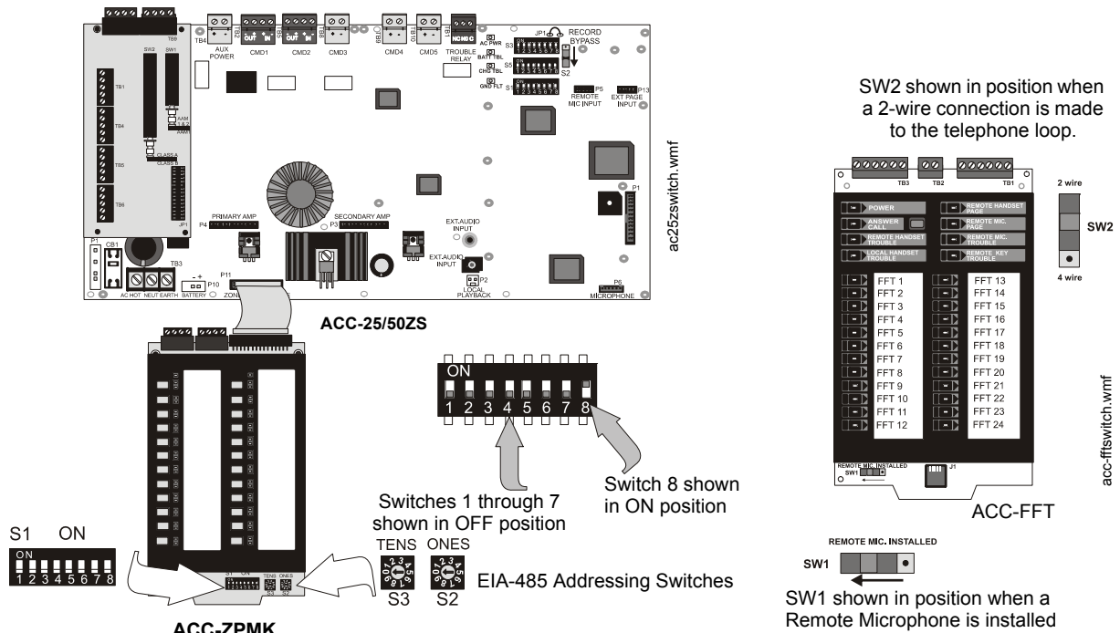
Figure 2.2 Field Programming DIP Switch for ACC-25/50ZS & ACC-25/50ZST Only
