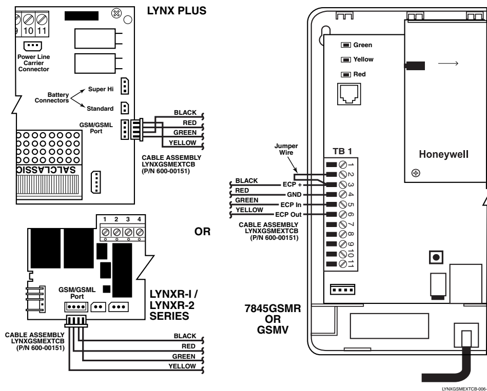
Figure 3. 7845GSMR or GSMV Connections
