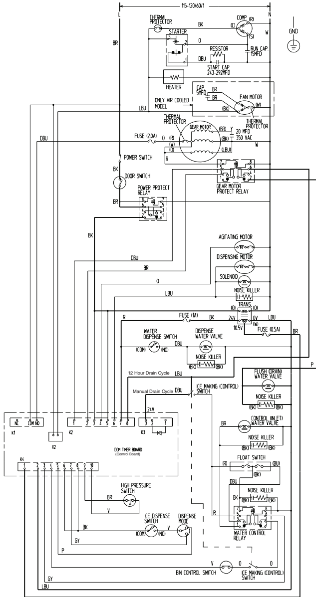
WIRING DIAGRAM
