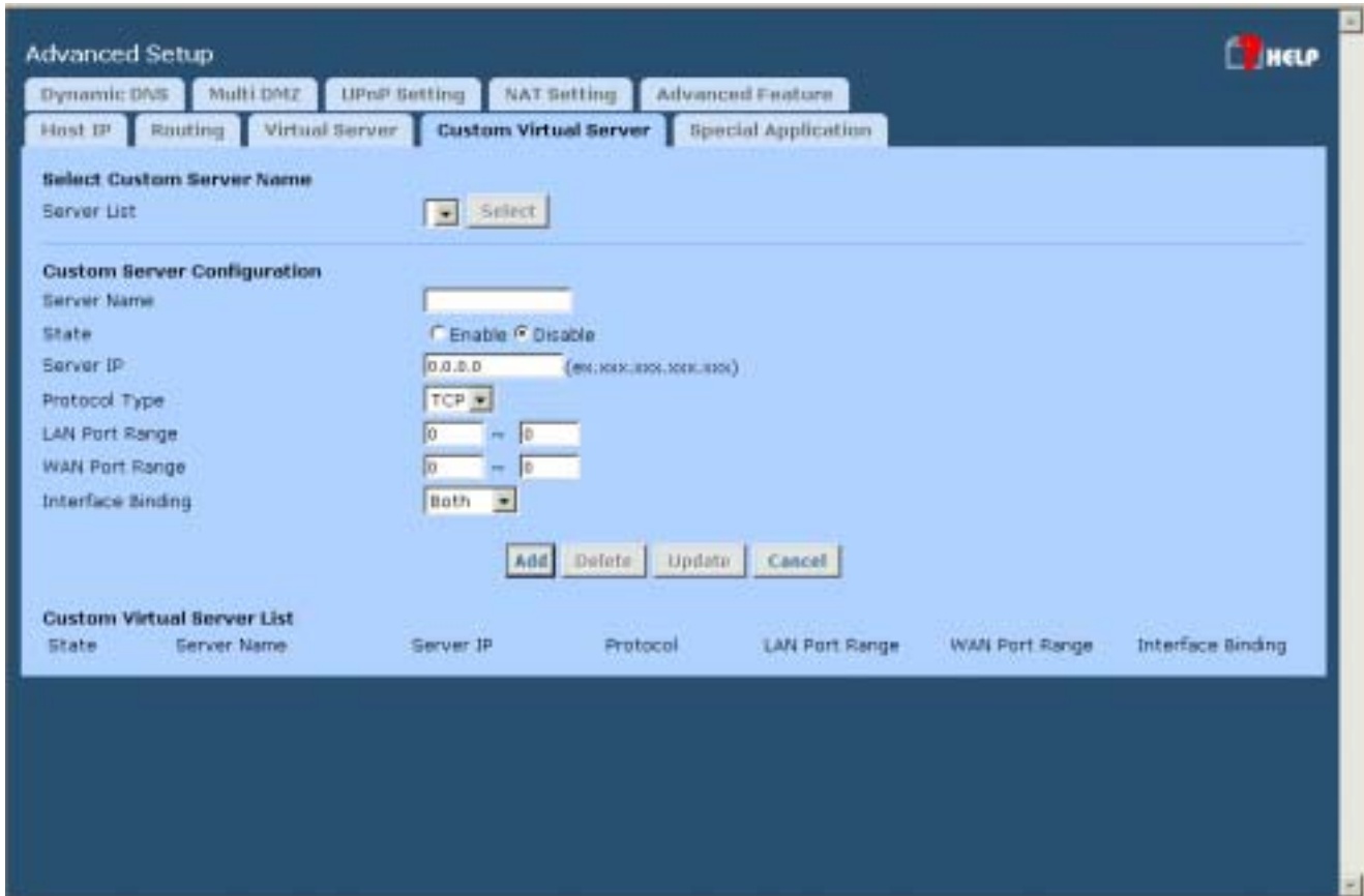
Figure 4-4: Custom Virtual Servers
