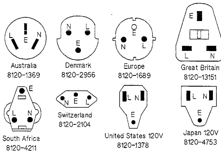
Figure 1-2. Power Cables - Plug Identification
