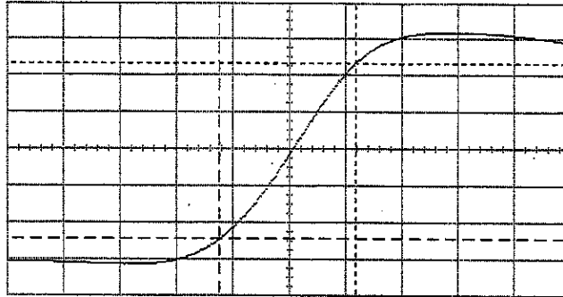
Figure 6-19. Risetime 10-90%
