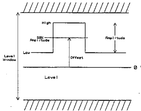
Figure 4-1. Output Levels: Amplitude, Offset, High- and Low-levels.
