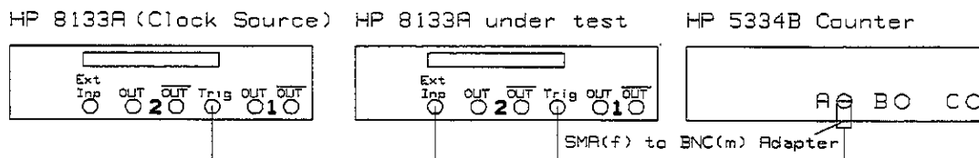
Figure 6-2. External Frequency Counter Low Frequency Test Set-up
