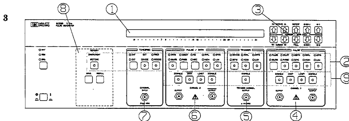
Figure 3-1. HP 8133A Frontpanel overview
