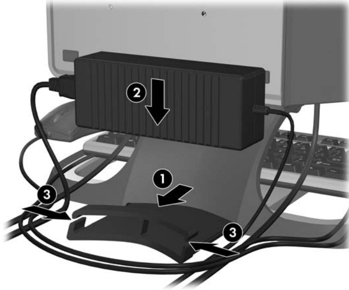
Figure 3-9 Installing the Power Supply
