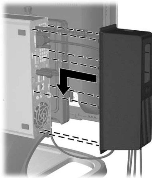
Figure 3-8 Installing the Port Cover
