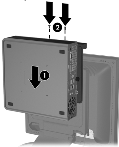
Figure 3-6 Sliding the USDT onto the Stand
