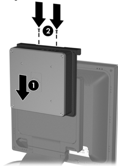
Figure 3-14 Sliding the Thin Client onto the Stand
