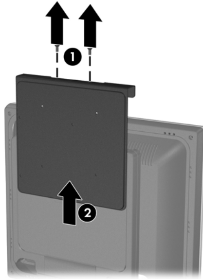
Figure 3-4 Removing the Computer Mounting Bracket
