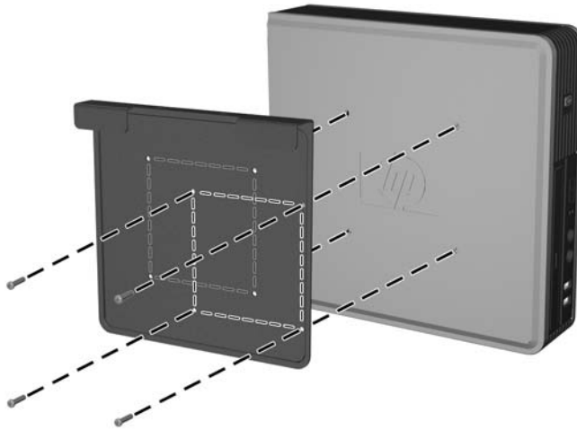
Figure 3-5 Installing the Computer Mounting Bracket on the USDT
