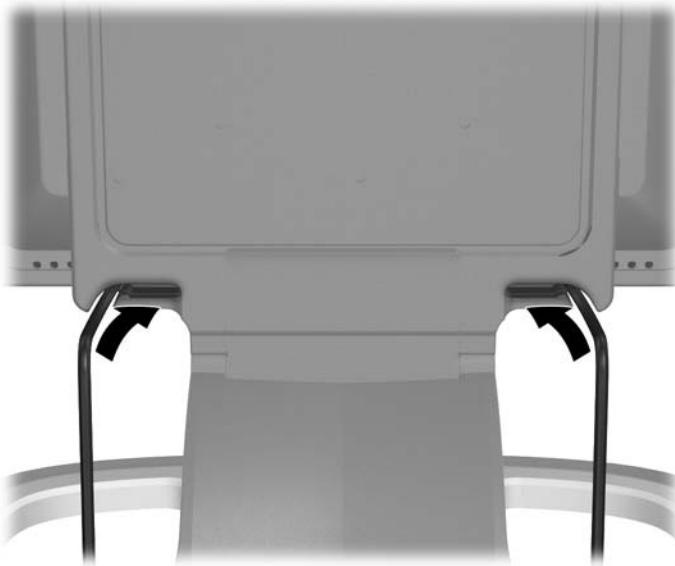
Figure 3-3 Routing Monitor VGA and Power Cables
