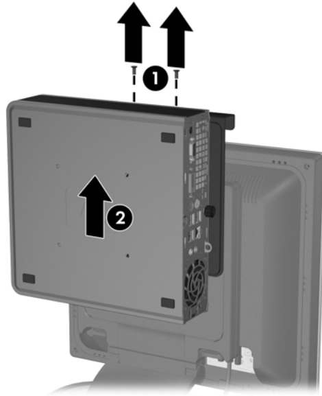
Figure 3-21 Removing the Computer from the Stand (USDT Computer Shown)
