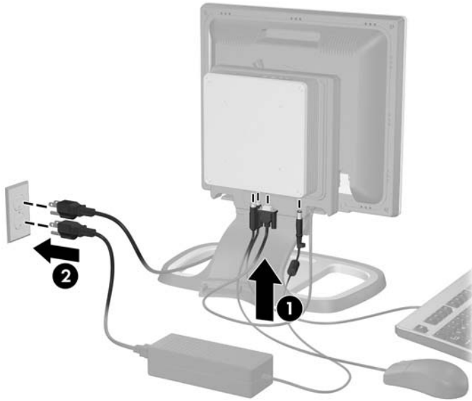
Figure 3-15 Connecting the Cables
