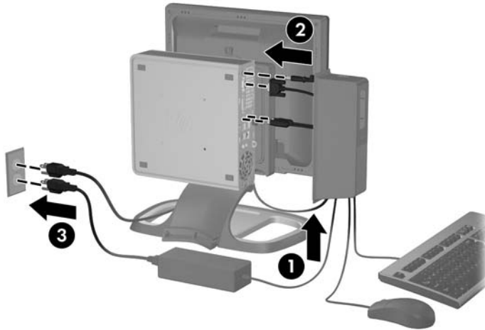
Figure 3-7 Connecting the Cables
