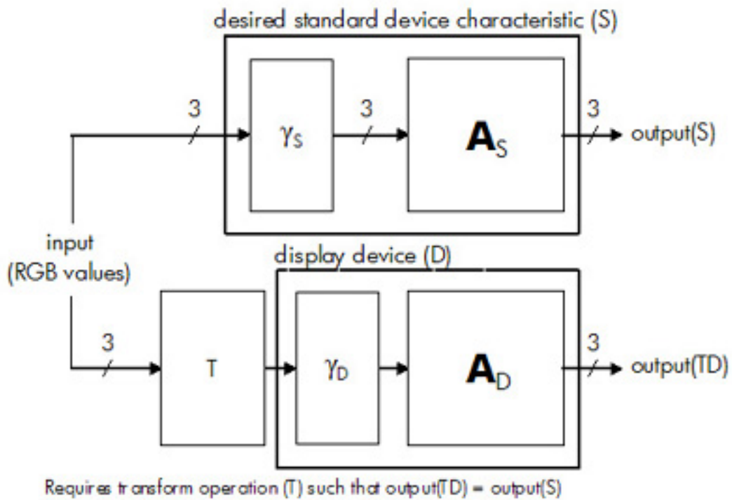
Figure A-4 Correcting Native Display Characteristics
