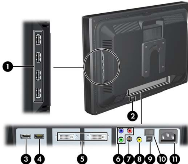
Figure 3-2 Rear Components
