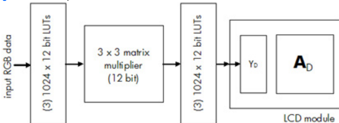
Figure A-5 Color Space Conversion Hardware in the LP2480zx
