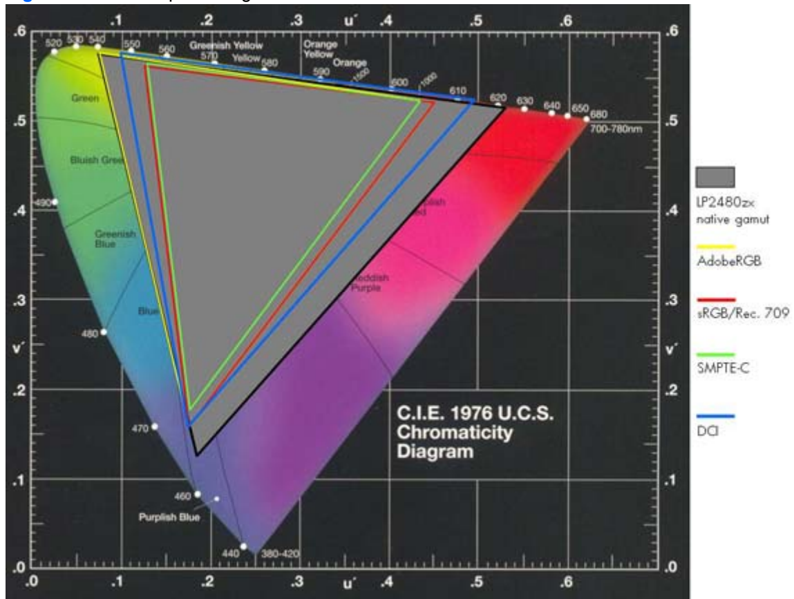
Figure A-1 Color Space Diagram
