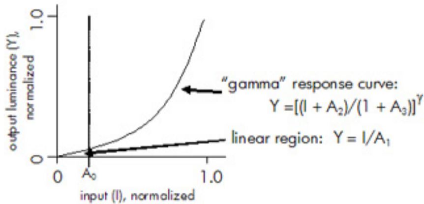
Figure A-7 Low Linear Region Response Curve
