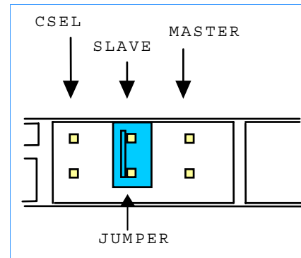
Figure 7 Drive Jumpers
