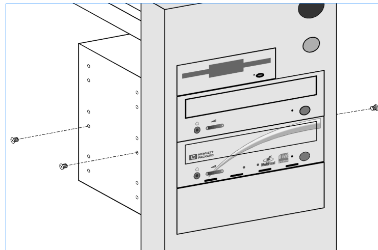
Figure 25 Securing the Drive in the Bay
