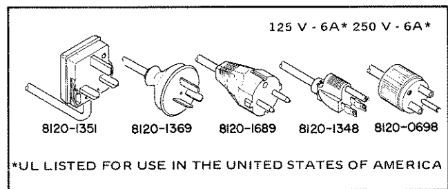
Figure 2-2. Power Cords.
