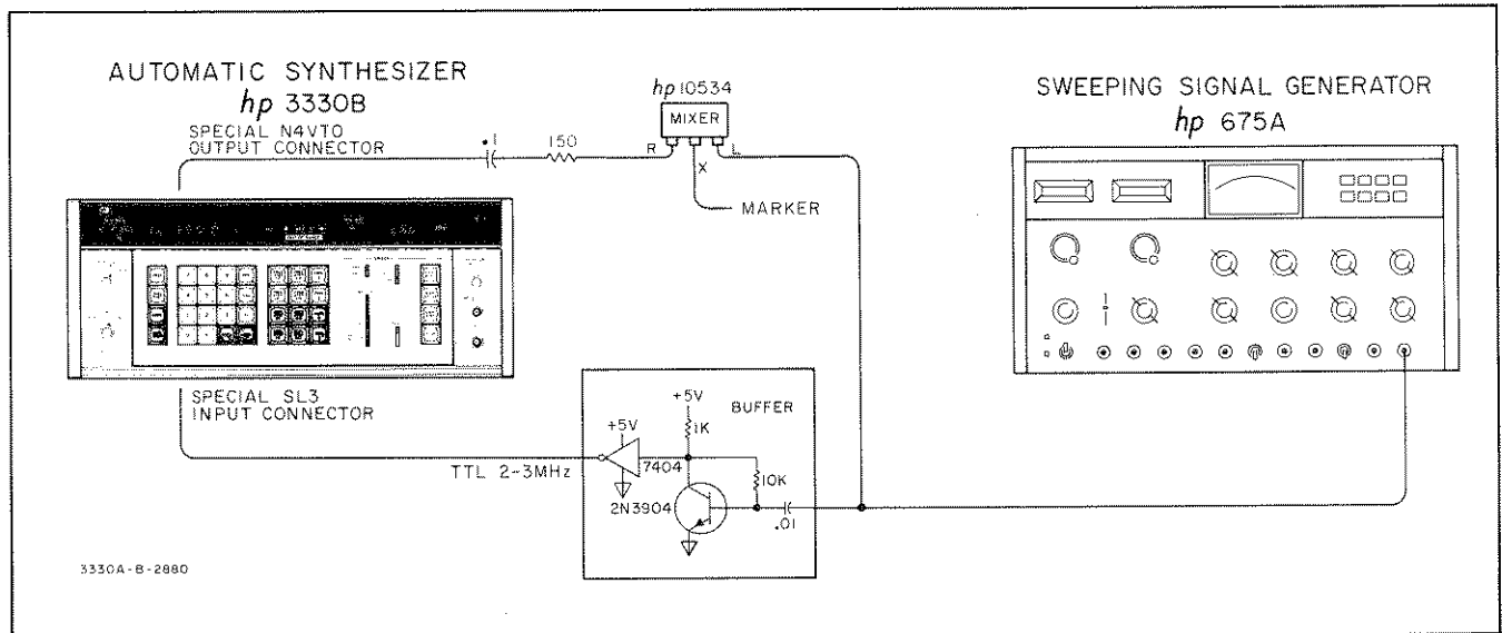
Figure 3-5. Special N4 Loop and SL3 Loop Connectors.
