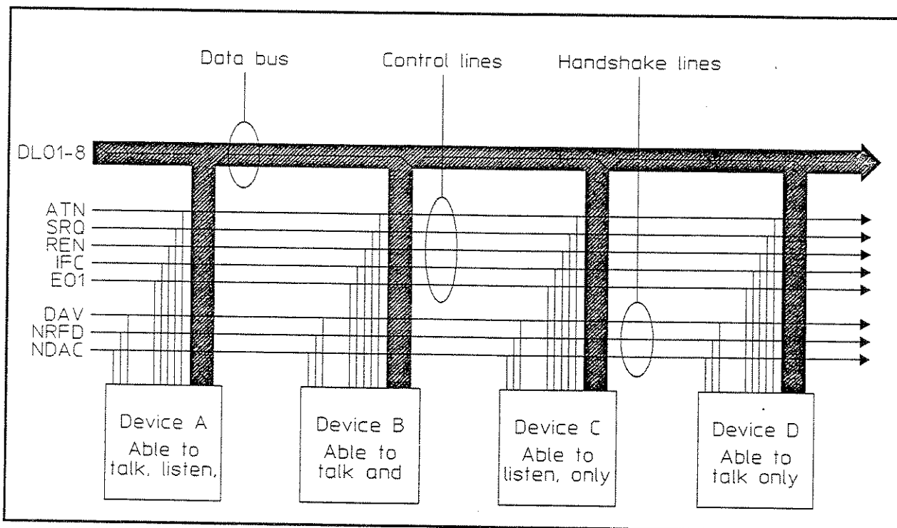
Figure 2-1. HP-IB Structure
