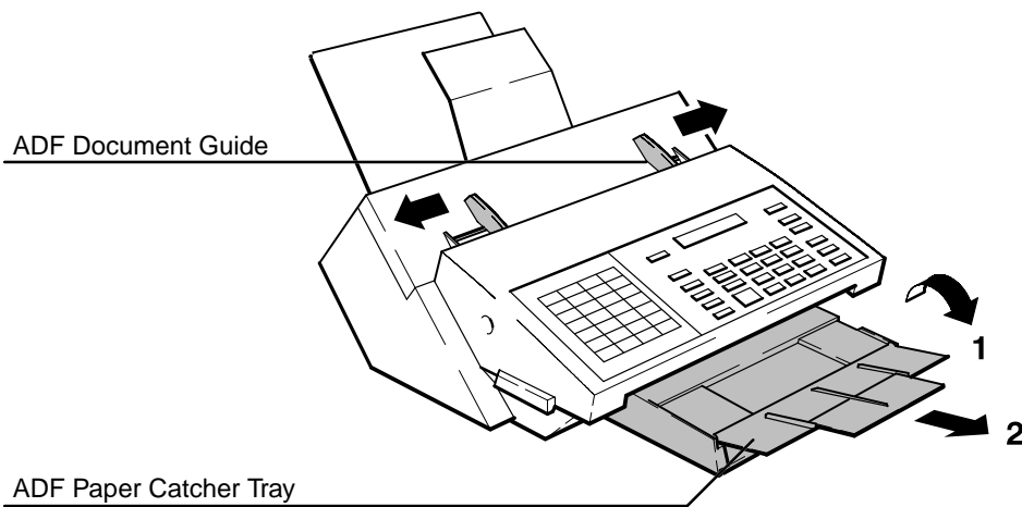
Figure 2-22. ADF Paper Catcher Tray Installation
