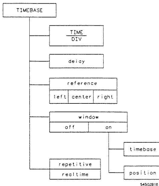
Figure 4-1. Timebase Menu
