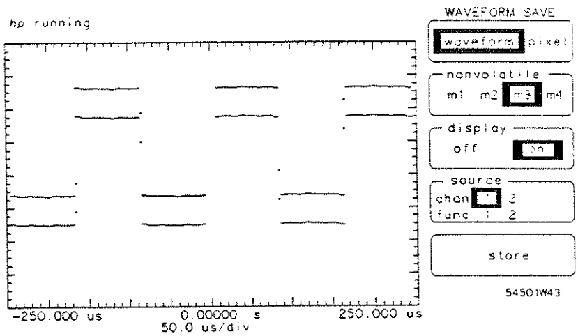
Figure 10-2. Displayed Memory
