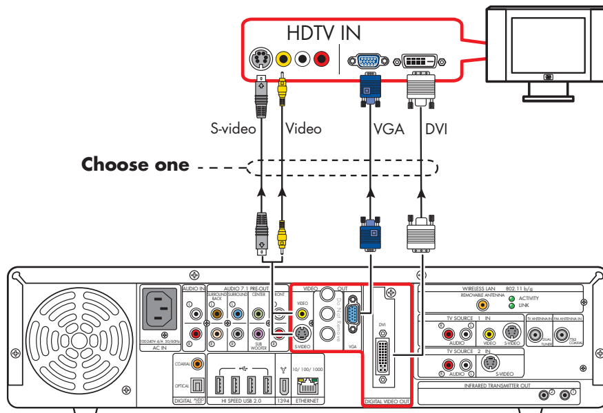
Video out to high-definition capable HDTV
