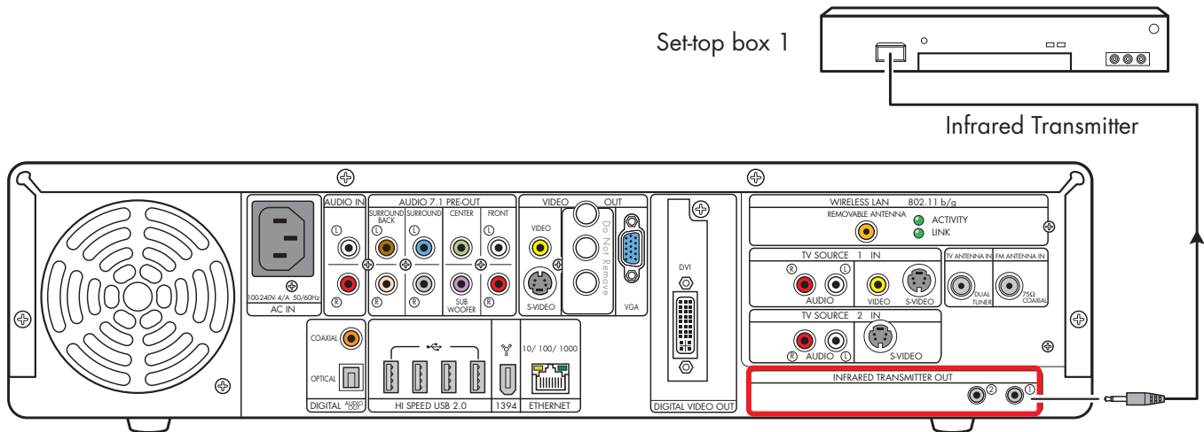
Infrared Transmitter connection (one set-top box)
