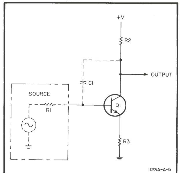
Figure 4-5. Miller Effect
