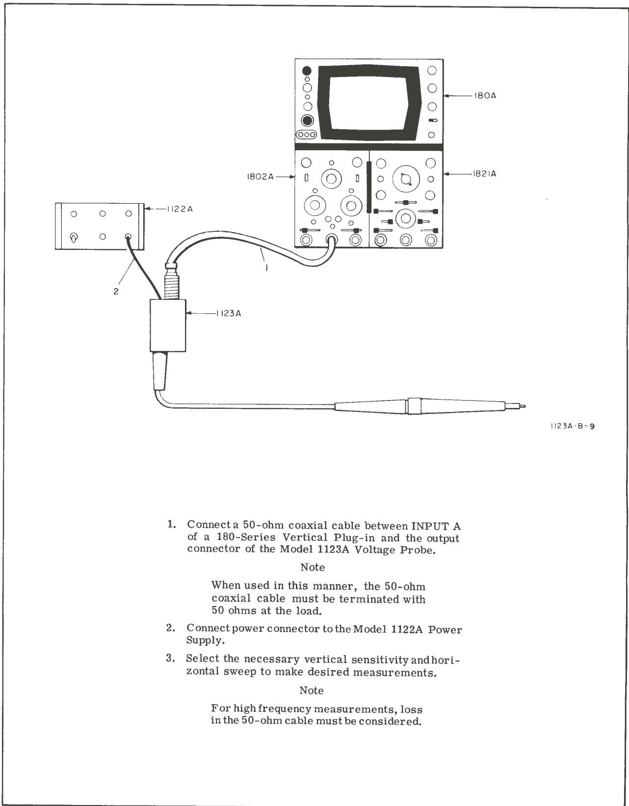
Figure 3-3. Remote Operation
