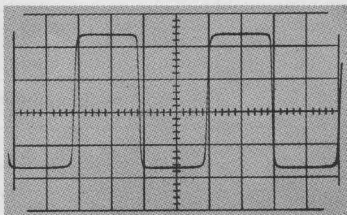
Figure 5-2. Approximate Chopper Waveform
