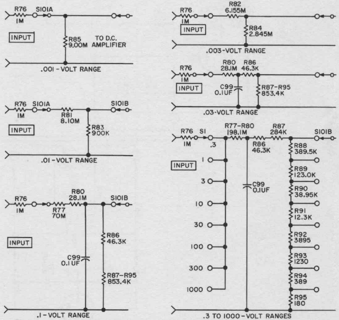
SIMPLIFIED DIAGRAM OF S101A & S101B SWITCHING
