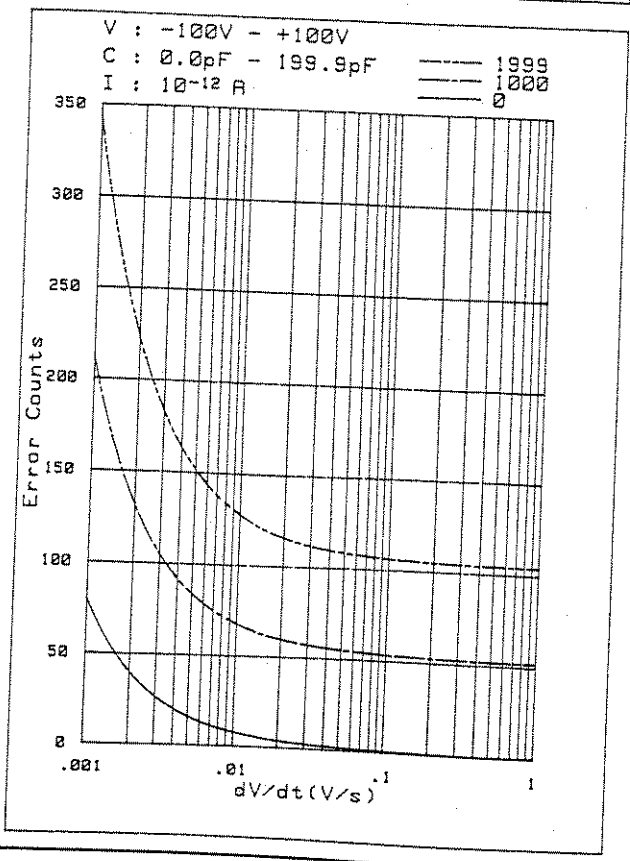
Figure 3-22. C-V Measurement Accuracy (Sheet 3 of 4).
