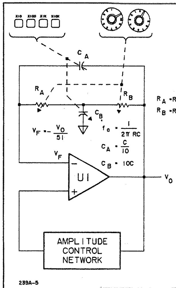
Figure 8-2. Simplified Oscillator Circuitry.
