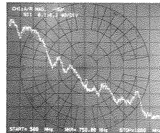
Passband Ripple at 0.01 dB/division using x10 magnification.
