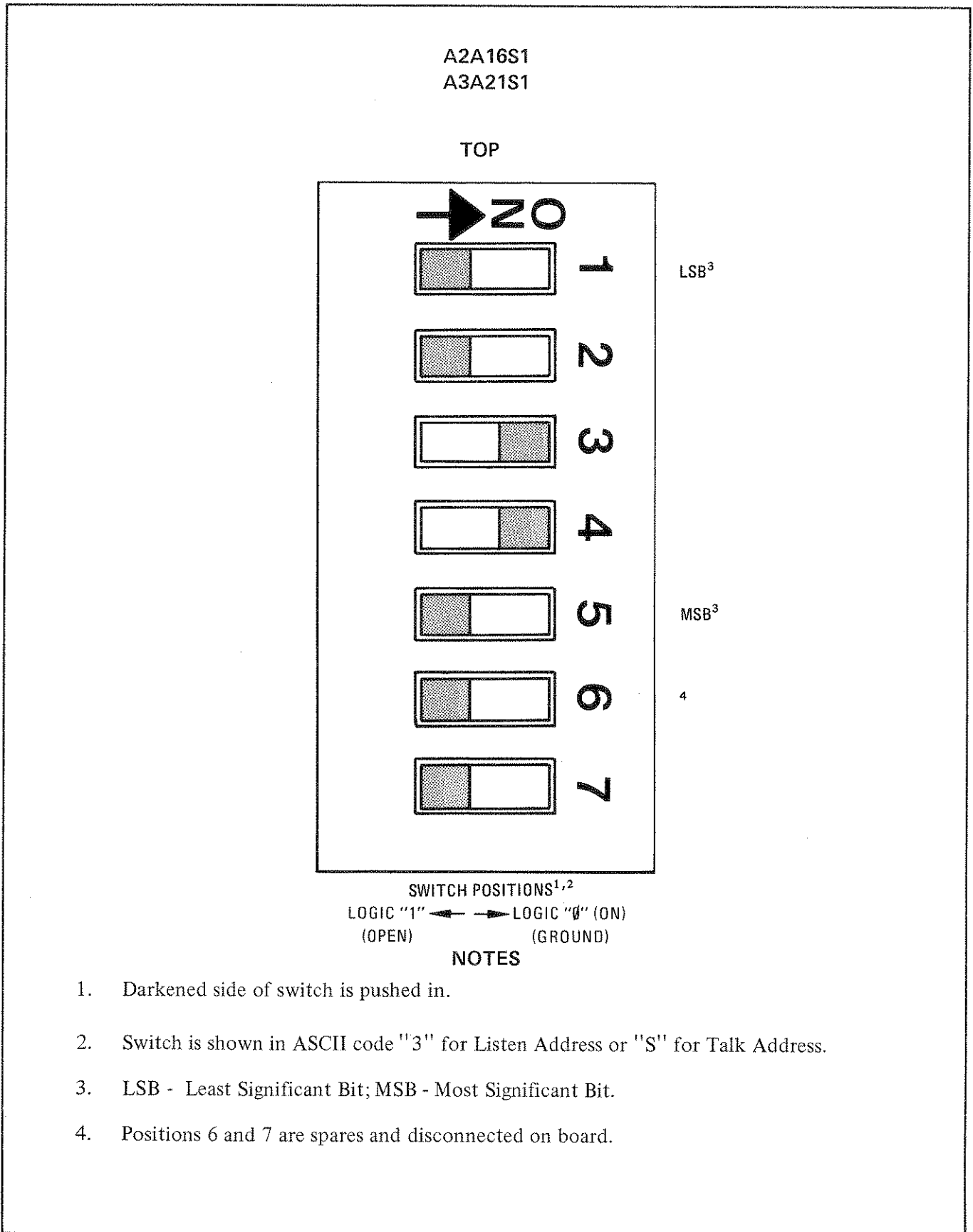
Figure A2-4. HP-IB Address Switch
