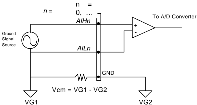
Figure 4.2.2 Ground source and differential input
