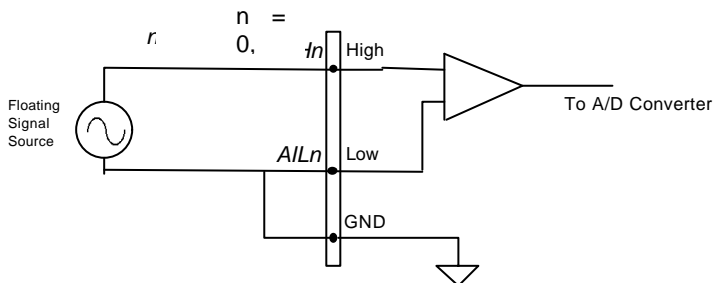
Figure 4.2.4 Floating source and differential input
