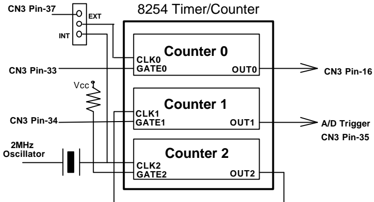
Figure 4.5 Block Diagram of 8254 Timer/Counter
