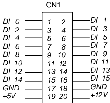
Figure 2.9.2 Pin Assignment of CN1
