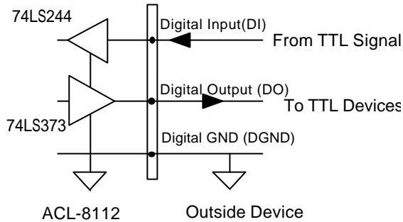
Figure 4.4 Digital I/O Connection
