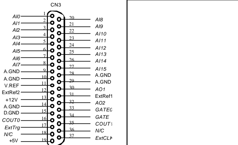
Figure 2.9.1 Pin Assignments of CN3
