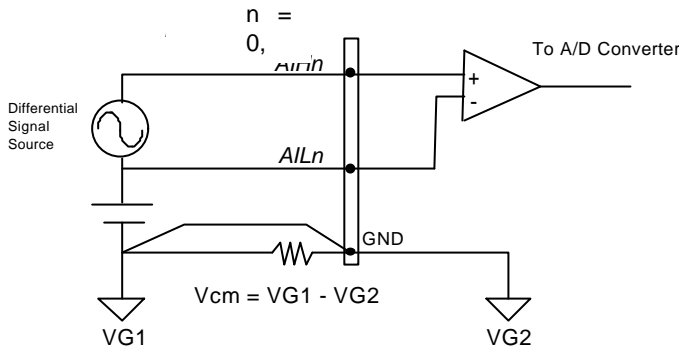
Figure 4.2.3 Differential source and differential input
