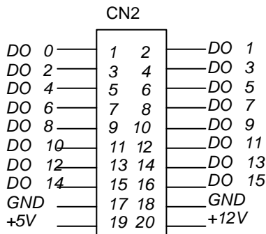
Figure 2.9.3 Pin Assignment of CN2
