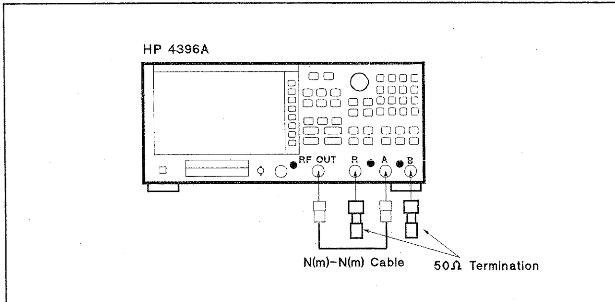
Figure 2-8. Input Crosstalk Test Setup 2
