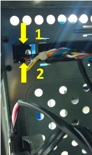
Figure 5-8 Removing the power switch/LED assembly
