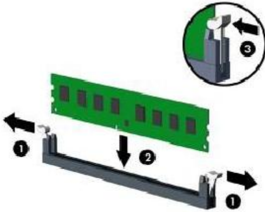
Figure 5-2 Installing a DIMM
