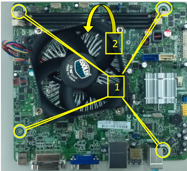
Figure 5-9 Removing the system board
