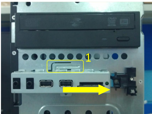
Figure 5-7 Removing the front I/O assembly
