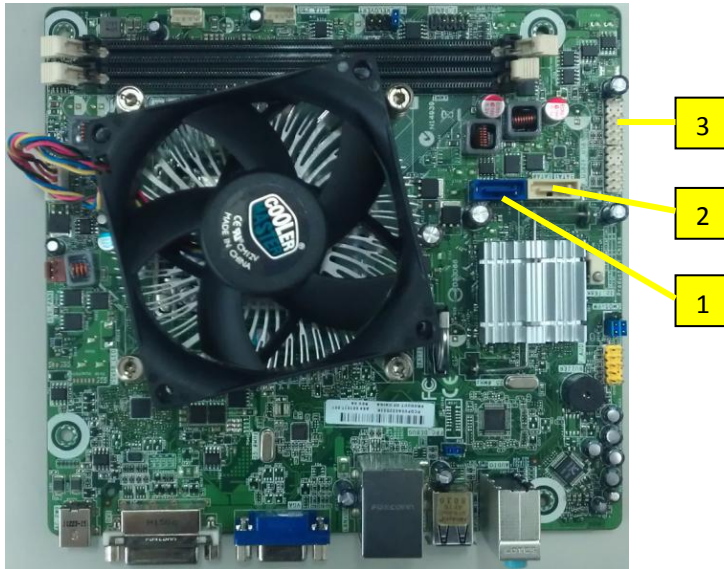
Figure 5-4 System Board Drive Connections –600B MT PC
