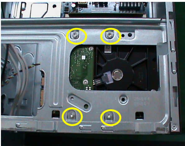
Figure 5-6 Hard drive cage screw location
