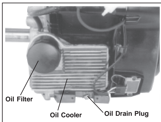
Figure 8. Oil Drain Plugs, Oil Filter, and Oil Cooler (CH25 shown).
