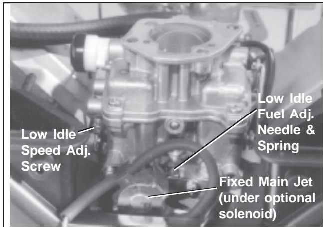
Figure 13. Carburetor (CH18-25).
