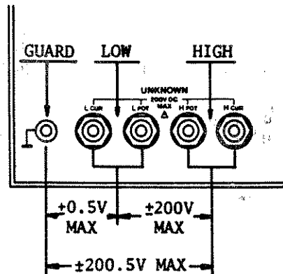
Interterminal Bias Limitations
