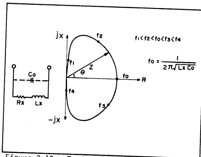
Figure 3-13. Typical Impedance Locus of an Inductor.
