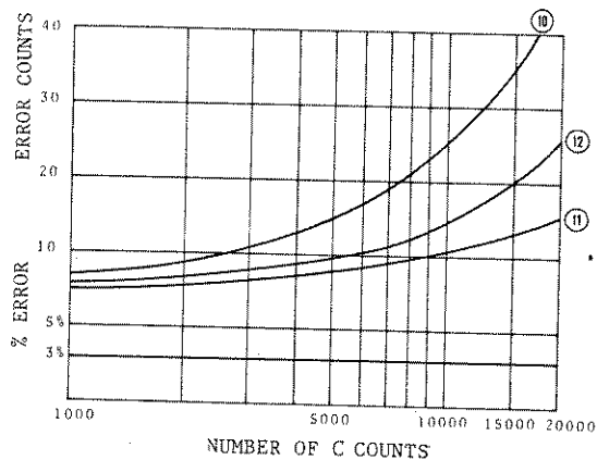
Figure 3-14. Measurement Accuracies (sheet 3 of 9).
