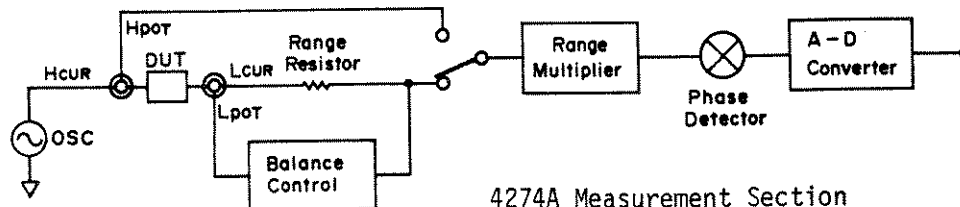
4274A Measurement Section
