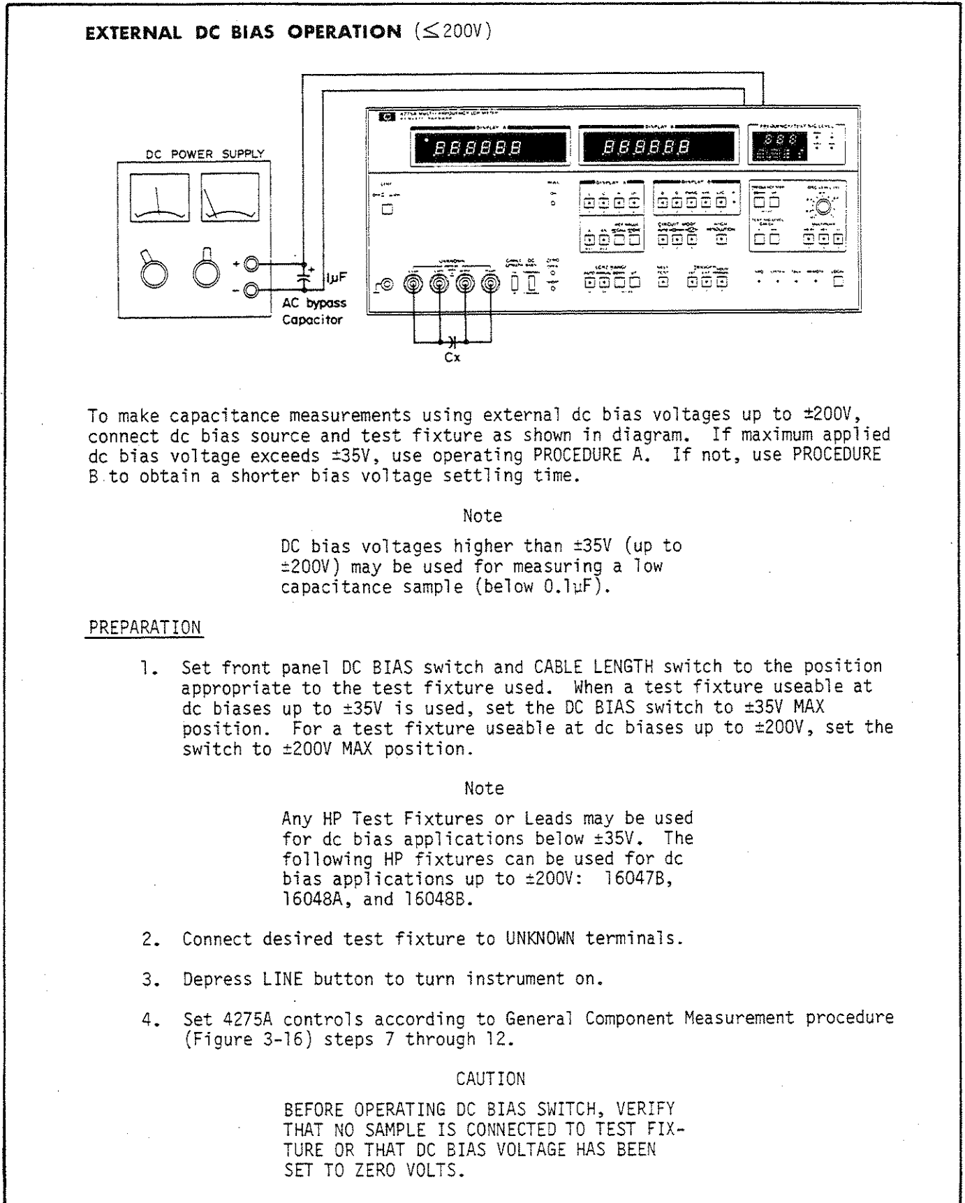
Figure 3-19. External DC Bias Circuits (sheet 1 of 4).
