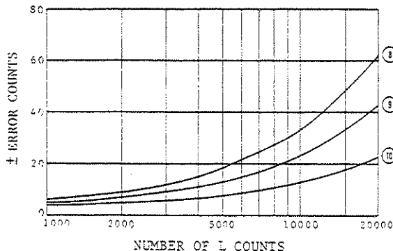
Figure 3-15. Measurement Accuracies (sheet 4 of 9).
