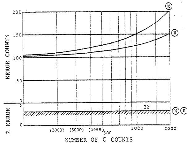
Figure 3-15. Measurement Accuracies (sheet 2 of 9).
