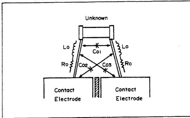
Figure 3-11. Parasitic Impedances Incident to DUT Connections.
