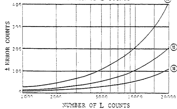
Figure 3-15. Measurement Accuracies (sheet 4 of 9).
