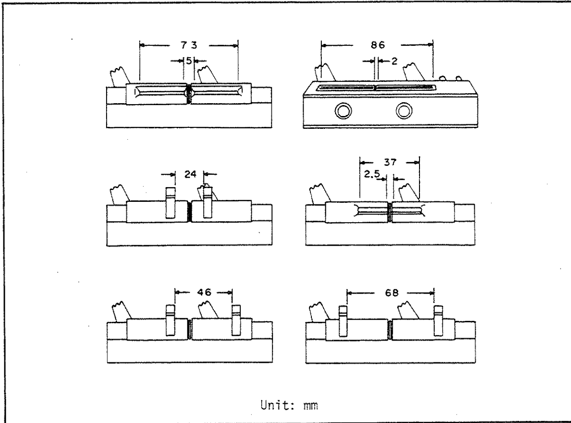
Figure 1-3. Dimensions of Test Fixture Contacts.
