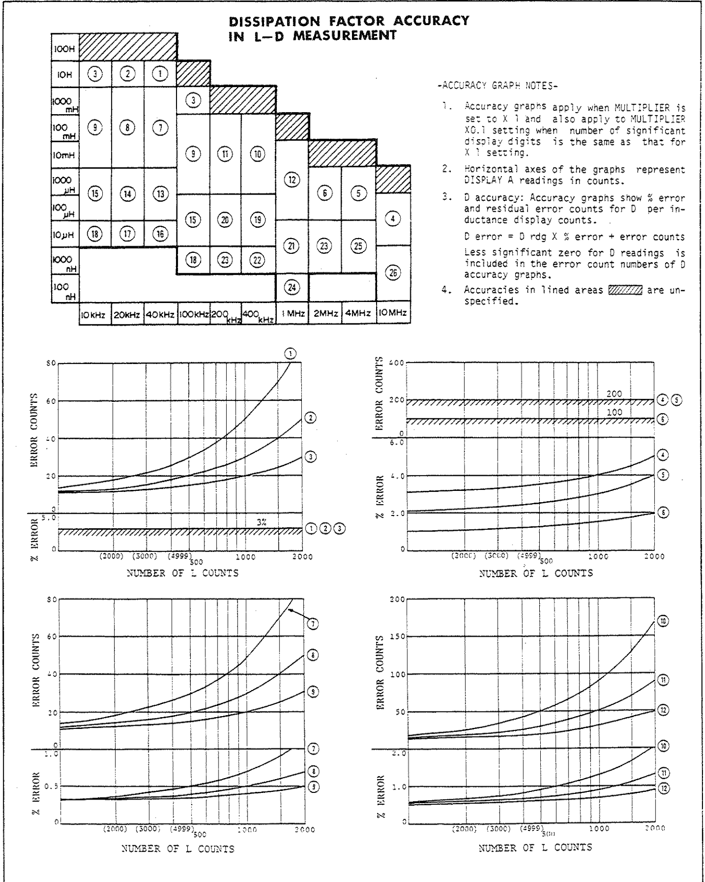
Figure 3-15. Measurement Accuracies (sheet 5 of 9).
