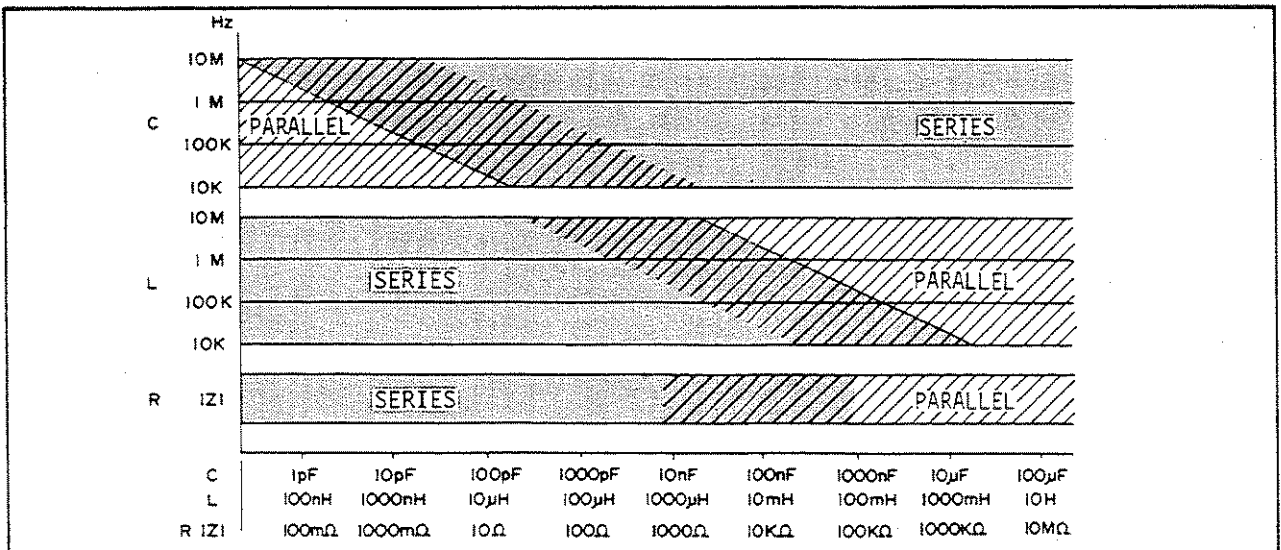
Figure 3-4. Approximate Relationships of Sample Values to Equivalent Circuit.
