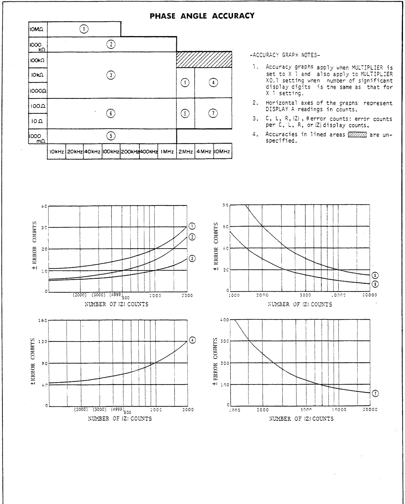
Figure 3-15. Measurement Accuracies (sheet 9 of 9).
