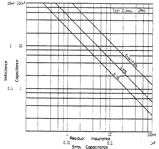
Figure 3-9. Relationships of Residual Parameters on Additional Errors.
