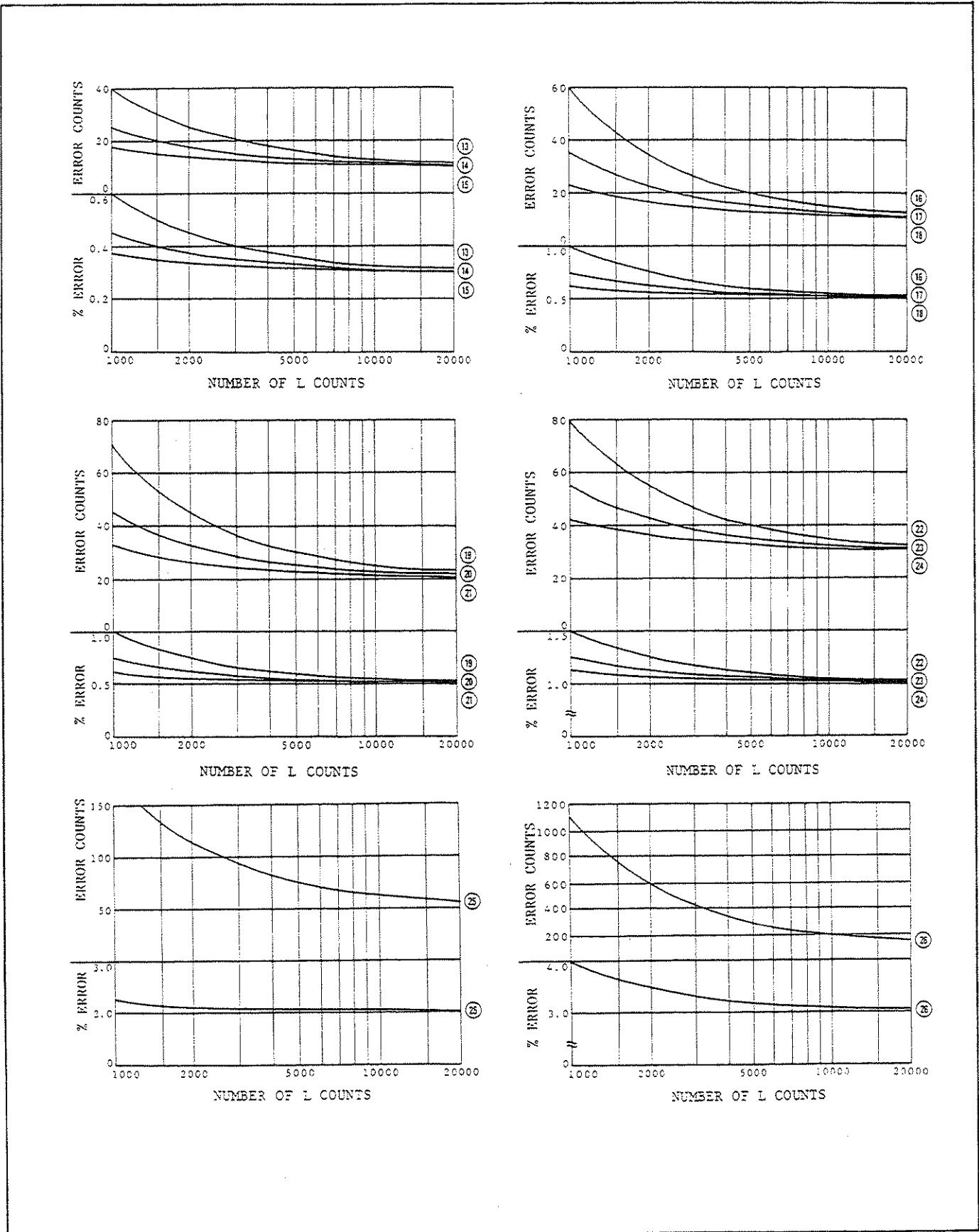
Figure 3-15. Measurement Accuracies (sheet 6 of 9).
