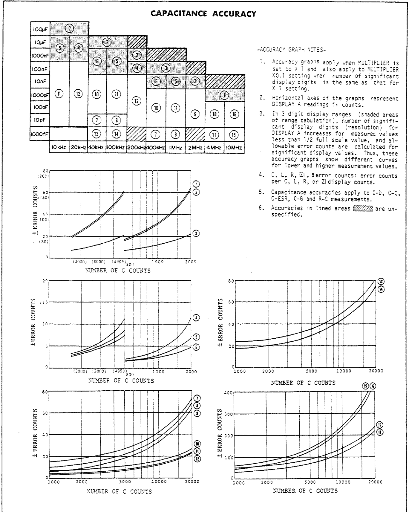
Figure 3-15. Measurement Accuracies (sheet 1 of 9).
