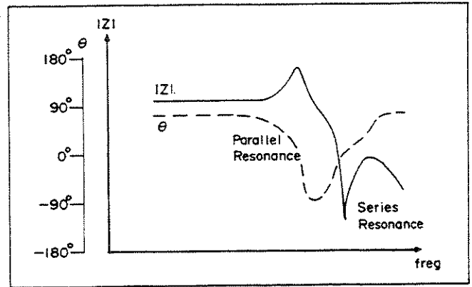
Figure 3-12. Effect of Resonance in sample (example).
