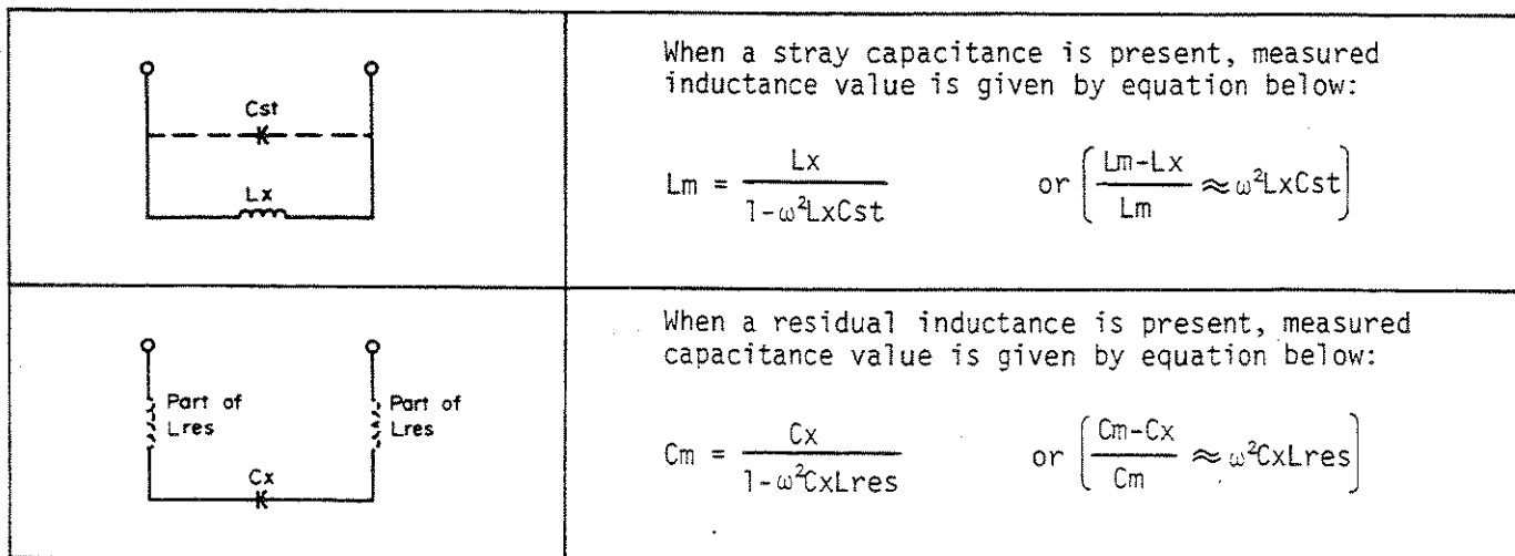
Figure 3-8. Residual Parameter Effects.
