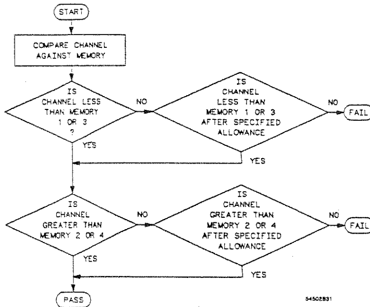
11-2. Waveform Comparison Test
