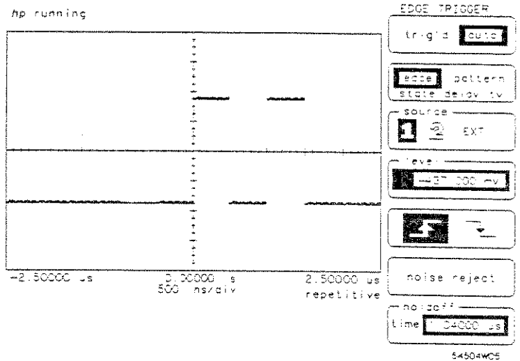
Figure 6-4. Two-Burst Pulse w/Stable Trigger
