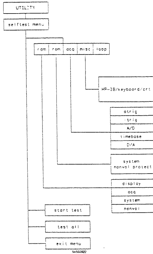
Figure 12-3. Self-Test Menu
