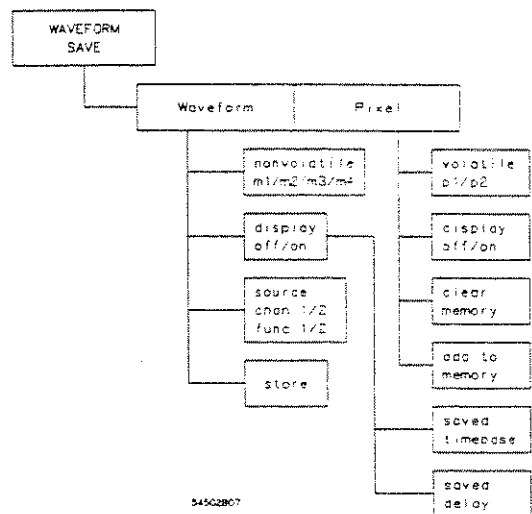
Figure 10-1. Waveform Save Menu
