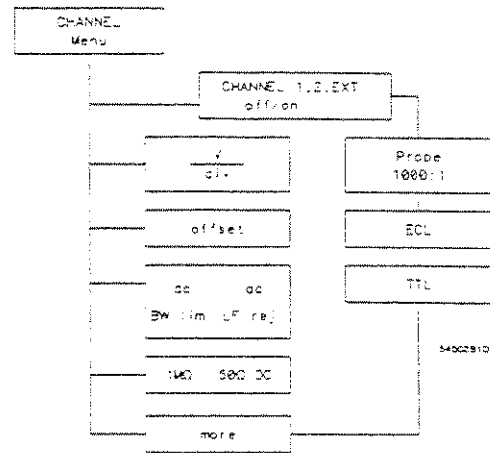
Figure S-1. HP 54510A Channel Menu
