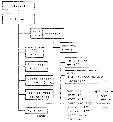
Figure 12-2. HP-IB Menu
