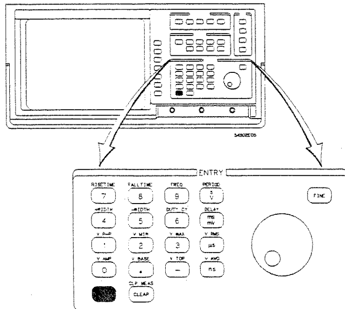
Figure 3-5. Entry Section
