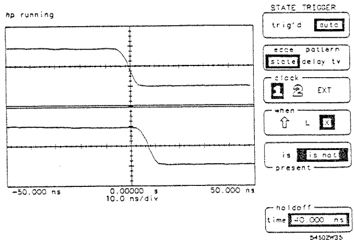
Figure 6-12. Channel 1 Clock LX State
