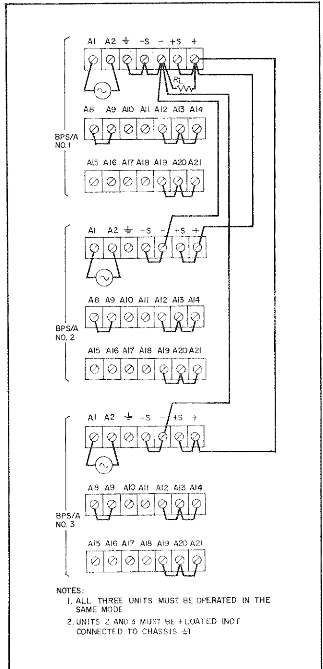
Figure 3-11. Parallel Connections
