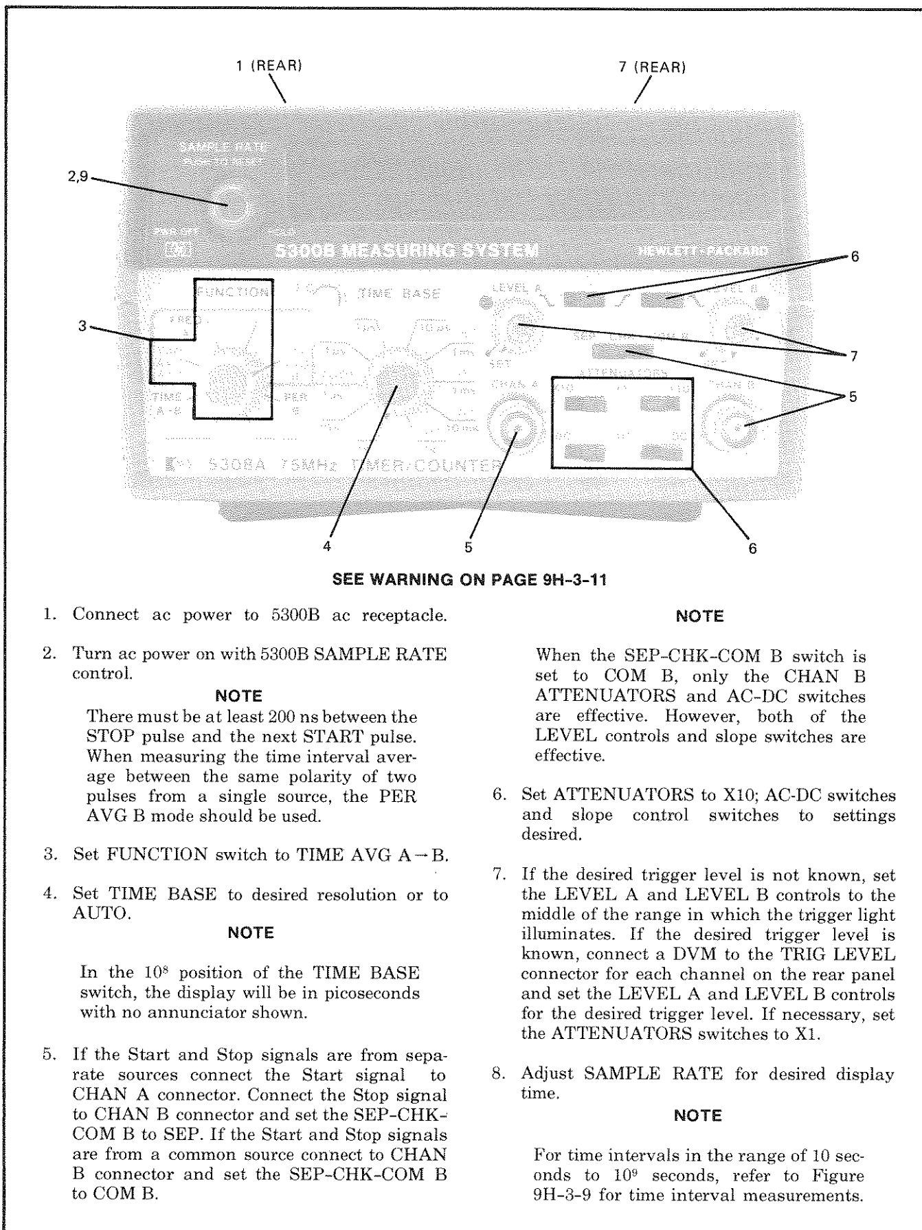
Figure 9H-3-10. Making Time Interval Average Measurements
